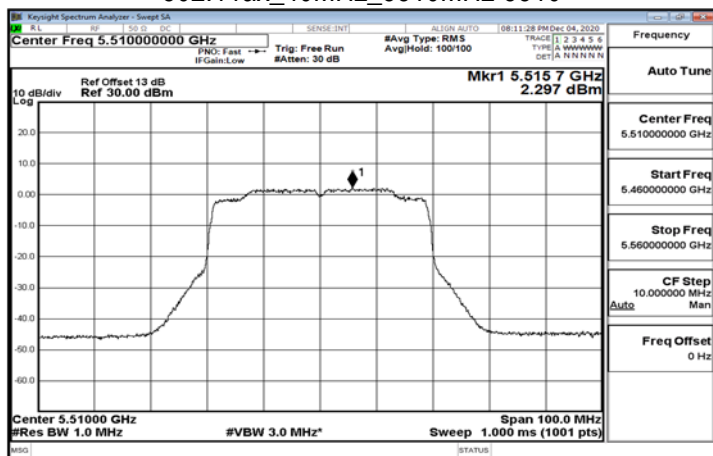
802.11ax_40MHz_5510MHz-5510
