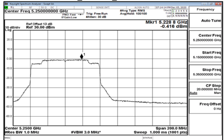
802.11ax_160MHz_5250MHz -996-S67
