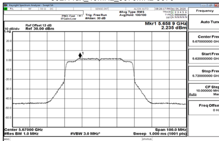
802.11ax_40MHz_5670MHz-5670
