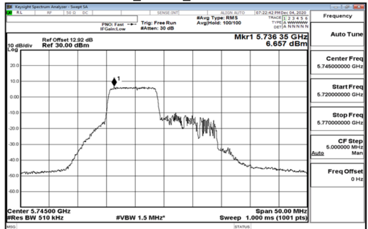
802.11ax_20MHz_5745MHz-26-0
