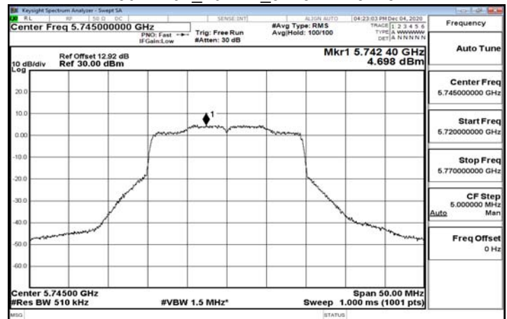
802.11ax_20MHz_5745MHz-106-53
