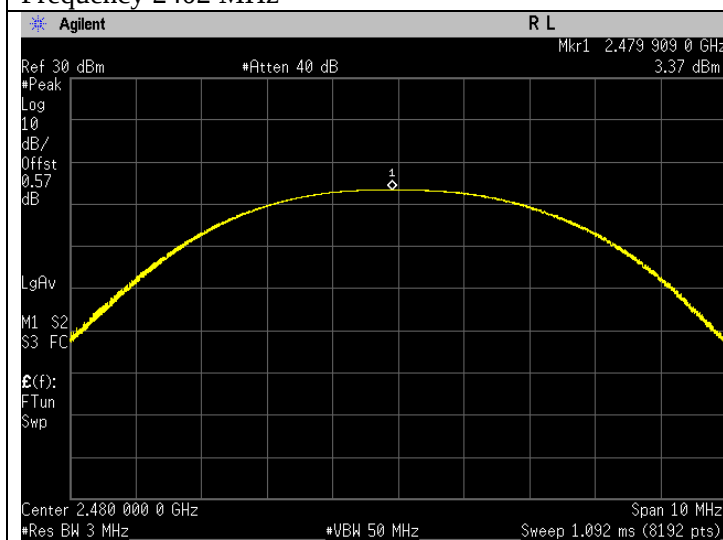
Frequency 2480 MHz
