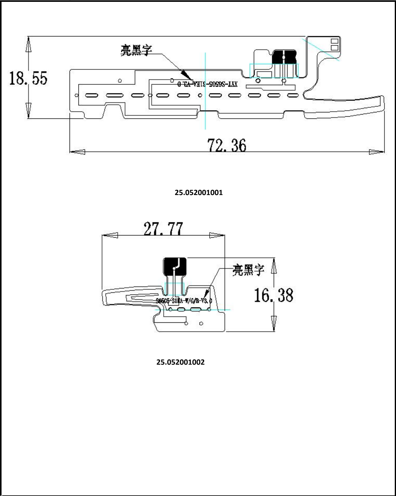
2D Product blueprint (DWG)
