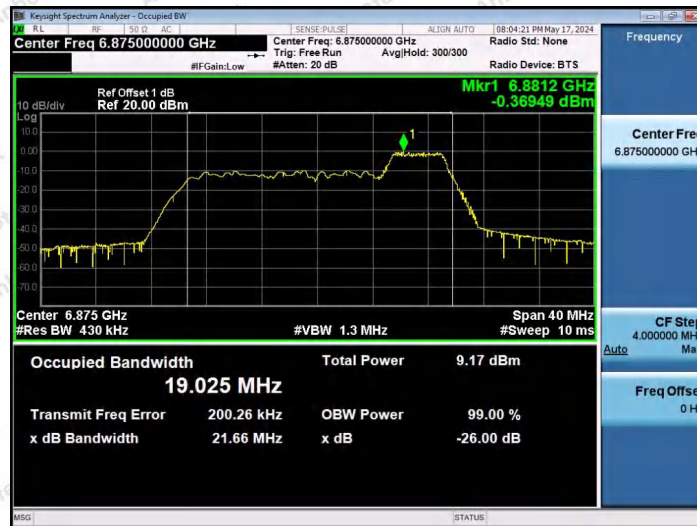
11AX20SISO-Ant1-6875-52Tone-RU40-PASS
