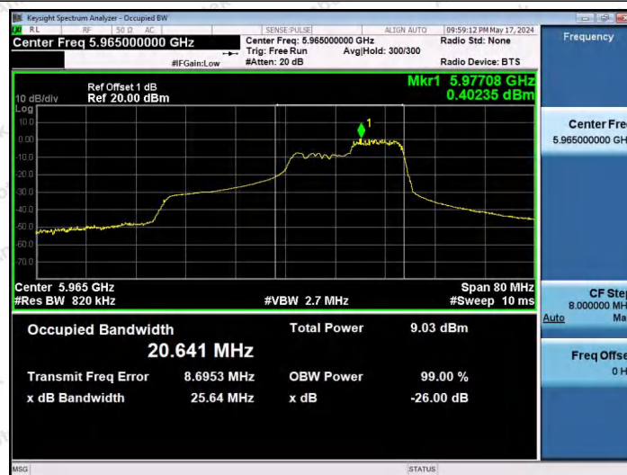
11AX40SISO-Ant1-5965-106Tone-RU56-PASS
