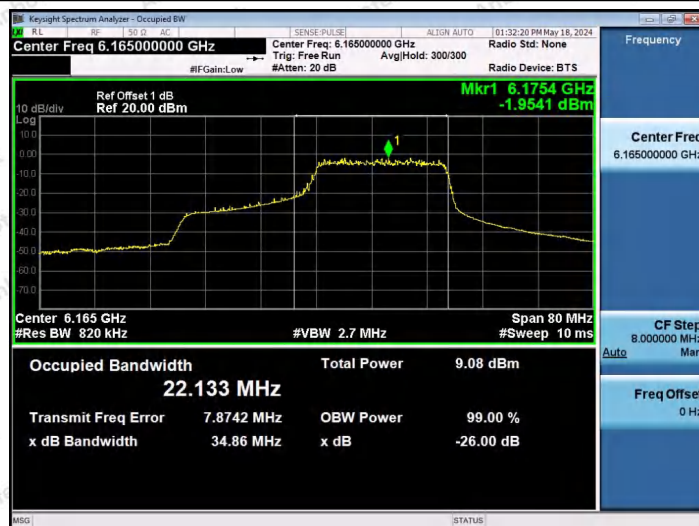
11AX40SISO-Ant1-6165-242Tone-RU62-PASS
