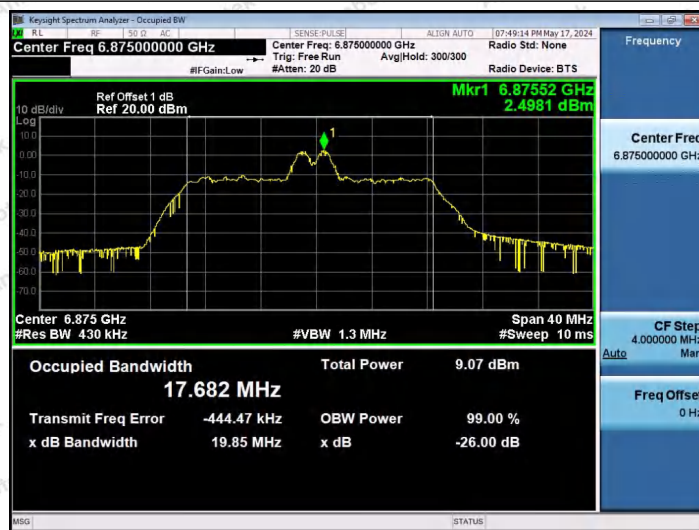
11AX20SISO-Ant1-6875-26Tone-RU4-PASS
