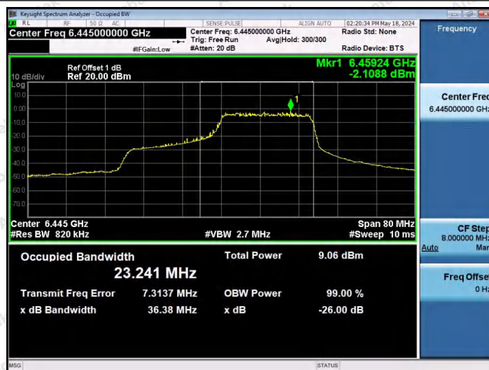
11AX40SISO-Ant1-6445-242Tone-RU62-PASS
