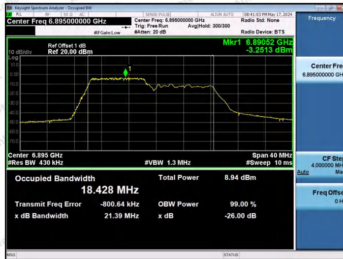
11AX20SISO-Ant1-6895-106Tone-RU53-PASS
