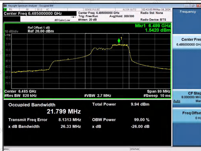
11AX40SISO-Ant1-6485-106Tone-RU56-PASS
