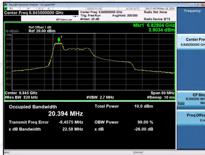
11AX40SISO-Ant1-6845-52Tone-RU37-PASS
