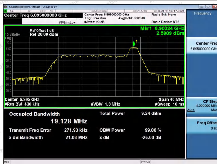
11AX20SISO-Ant1-6895-26Tone-RU8-PASS
