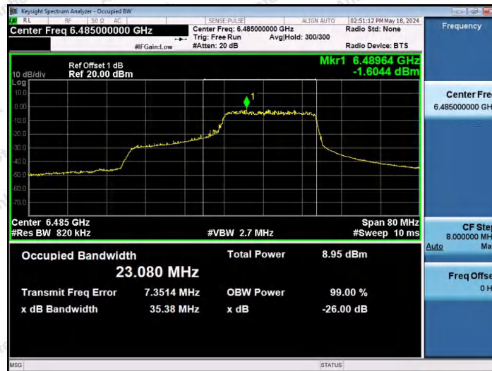
11AX40SISO-Ant1-6485-242Tone-RU62-PASS
