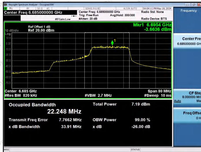
11AX40SISO-Ant1-6685-242Tone-RU62-PASS
