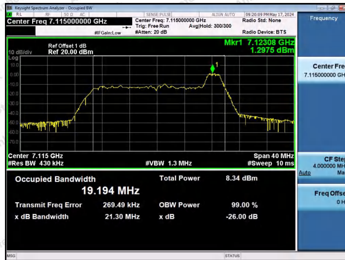
11AX20SISO-Ant1-7115-26Tone-RU8-PASS
