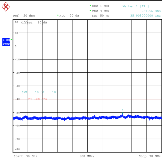
16QAM Low channel Full RB
