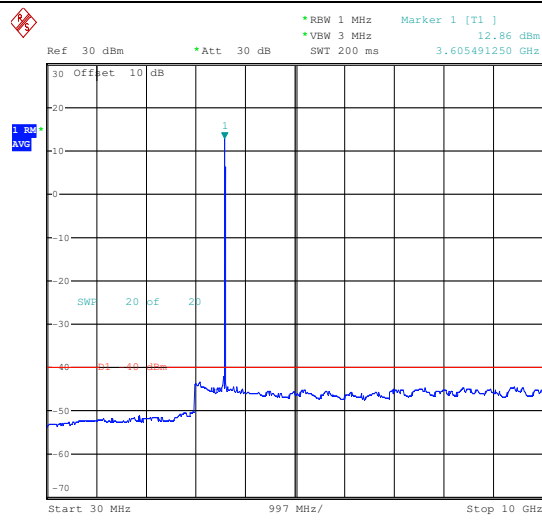
QPSK Middle channel Full RB
