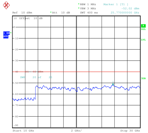
16QAM Low channel Full RB
