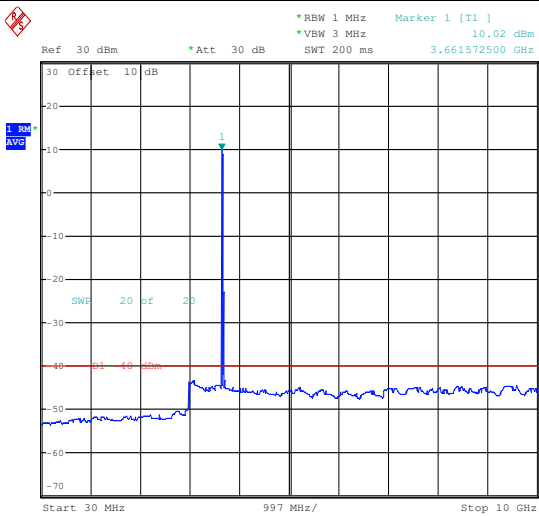
64QAM High channel Full RB
