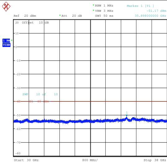
64QAM Low channel Full RB
