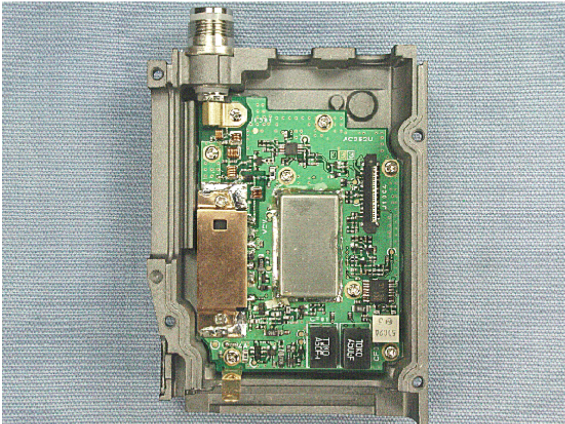
Internal view (rear)
