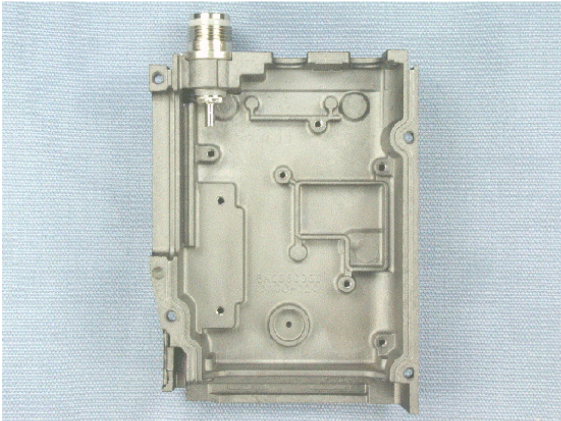
Inside of chassis (rear)
