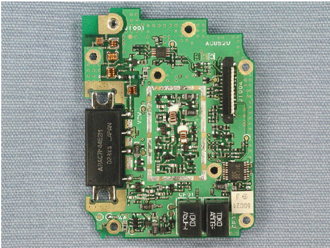
Side-A of RF-UNIT without shield case
