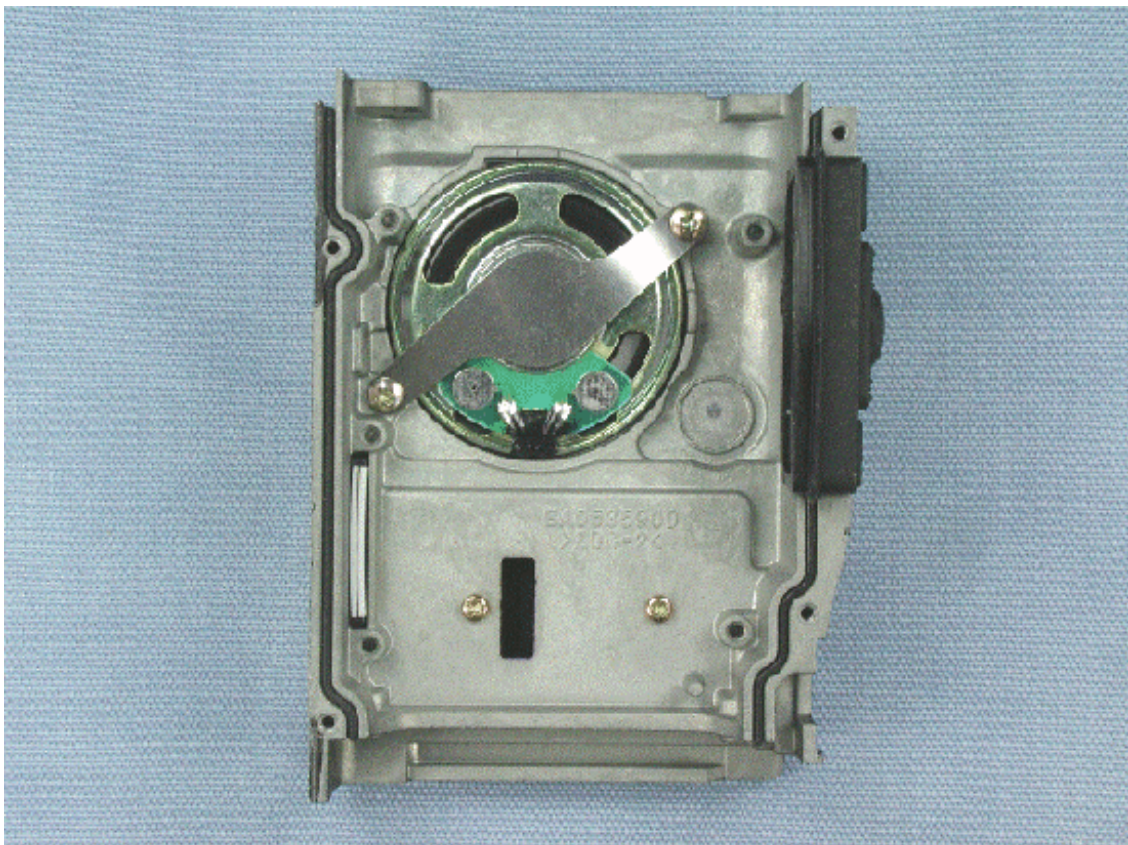
Inside of chassis (front)
