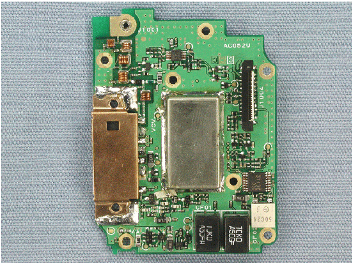
Side-A of RF-UNIT with shield case
