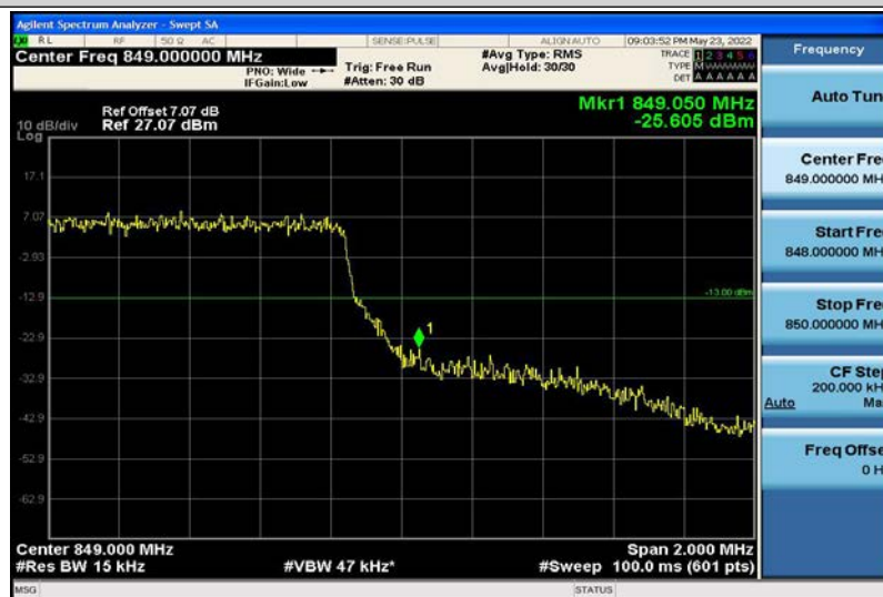
Band5-1.4MHz-16QAM-20643-6RB#0
