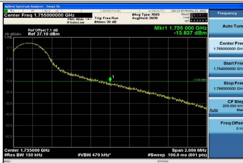
Band4-15MHz-16QAM-20325-1RB#74
