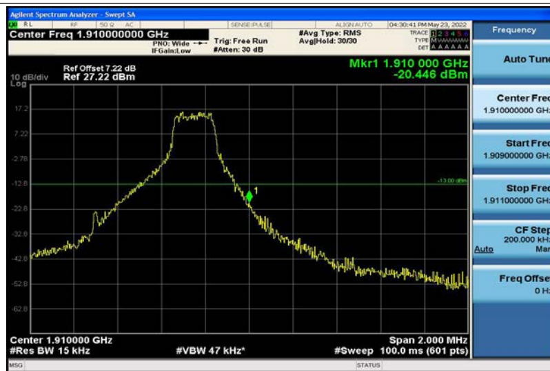
Band2-1.4MHz-16QAM-19193-1RB#5
