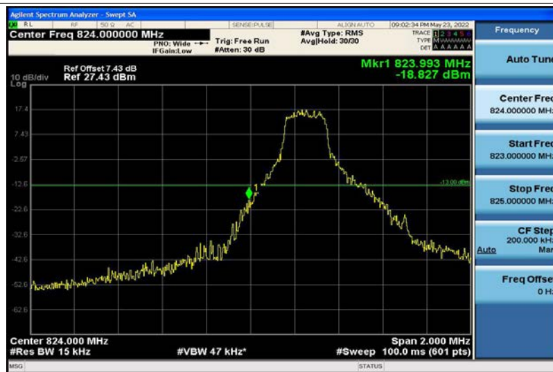
Band5-1.4MHz-QPSK-20407-1RB#0
