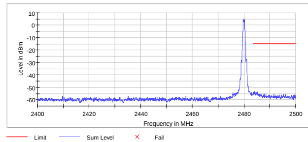
Figure 7.5.1.2-5: Upper Band-edge (1Mbps)
