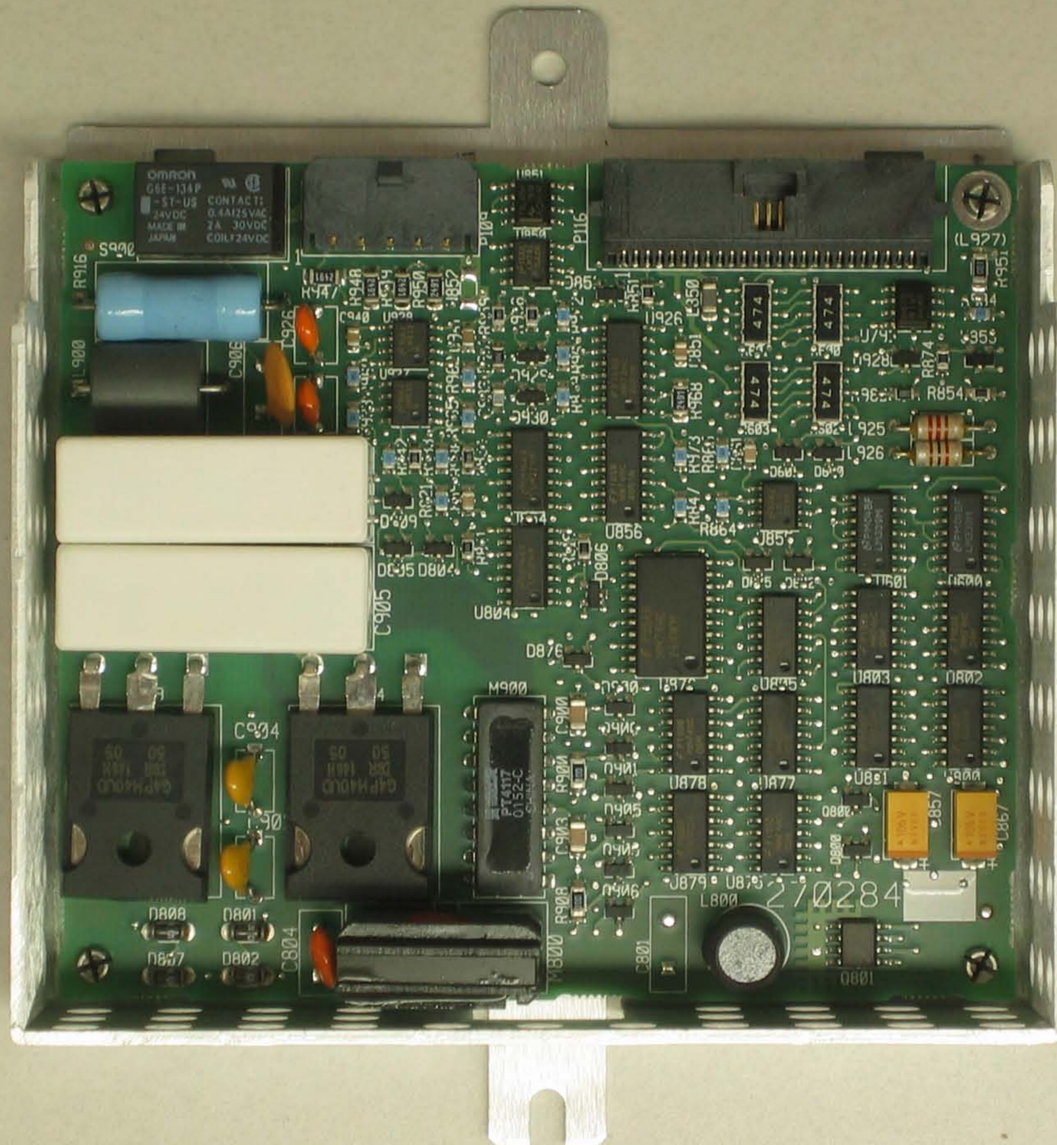
Inductive Telemetry Board Component Side
