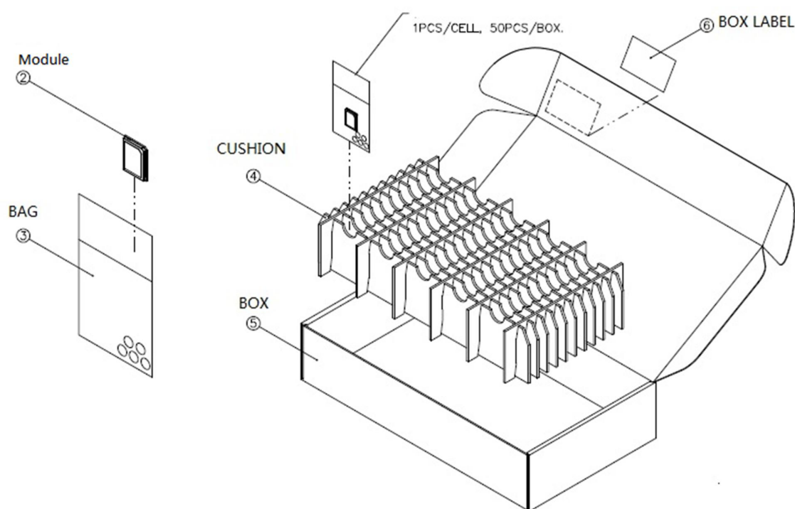
Figure 7-4. Packaging—carton
