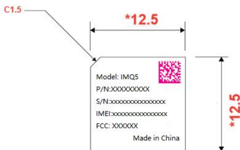
Figure 7-1. Label drawing
