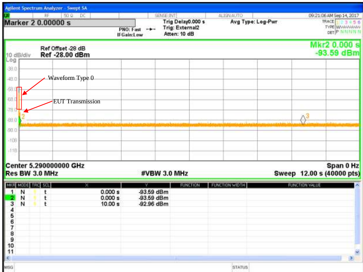
Figure 34: Channel Move Time and Channel Closing Transmission Time using Pulse Radar Waveform 0 in Master Mode 11AC VHT80, 80 MHz Bandwidth
