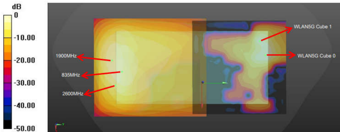
WWAN + WLAN 5GHz Back_5mm
