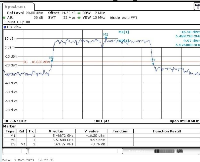
802.11ac VHT160MIMO Ant2 5570 MHz
