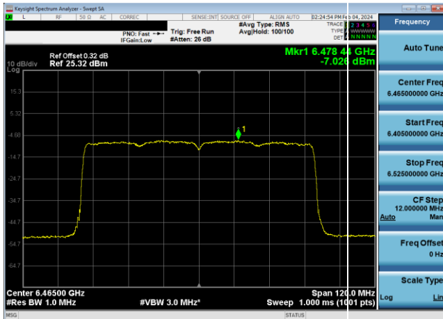
Plot 7-673. Power Spectral Density Plot SDM Diversity Antenna WF7 LPI (80MHz 802.11ax (UNII Band 6) – Ch. 103, MCS11)
