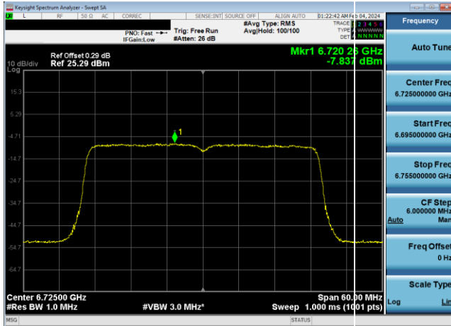
Plot 7-678. Power Spectral Density Plot SDM Diversity Antenna W8 LPI (40MHz 802.11ax (UNII Band 7) – Ch. 155, MCS11)
