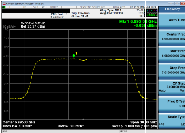
Plot 7-685. Power Spectral Density Plot SDM Diversity Antenna WF7 LPI (20MHz 802.11ax (UNII Band 8) – Ch. 209, MCS11)
