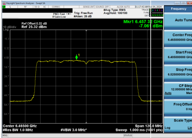
Plot 7-672. Power Spectral Density Plot SDM Diversity Antenna WF8 LPI (80MHz 802.11ax (UNII Band 6) – Ch. 103, MCS11)
