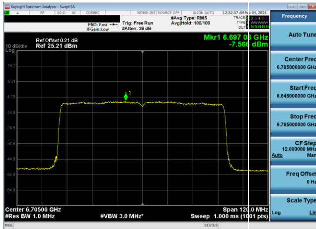
Plot 7-648. Power Spectral Density Plot SDM Diversity Antenna WF8 LPI (80MHz 802.11ax (UNII Band 7) – Ch. 151, MCS4)
