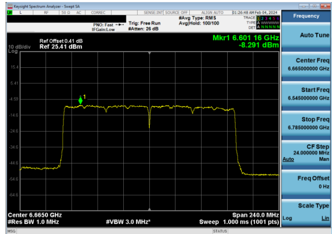
Plot 7-682. Power Spectral Density Plot SDM Diversity Antenna W8 LPI (160MHz 802.11ax (UNII Band 7) – Ch. 143, MCS11)
