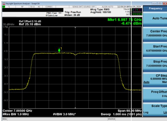
Plot 7-654. Power Spectral Density Plot SDM Diversity Antenna WF8 LPI (40MHz 802.11ax (UNII Band 8) – Ch. 211, MCS4)
