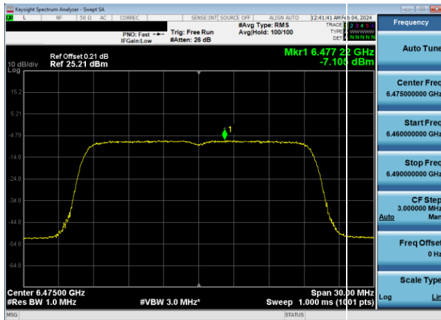
Plot 7-636. Power Spectral Density Plot SDM Diversity Antenna WF8 LPI (20MHz 802.11ax (UNII Band 6) – Ch. 105, MCS4)
