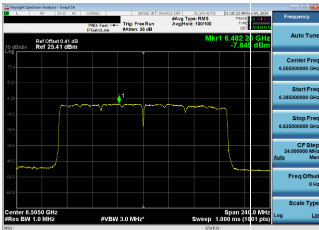
Plot 7-674. Power Spectral Density Plot SDM Diversity Antenna WF8 LPI (160MHz 802.11ax (UNII Band 6) – Ch. 111, MCS11)
