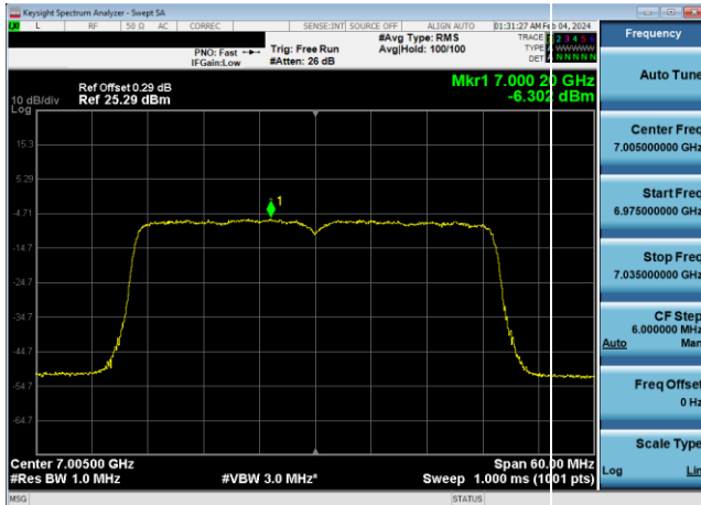
Plot 7-686. Power Spectral Density Plot SDM Diversity Antenna WF8 LPI (40MHz 802.11ax (UNII Band 8) – Ch. 211, MCS11)
