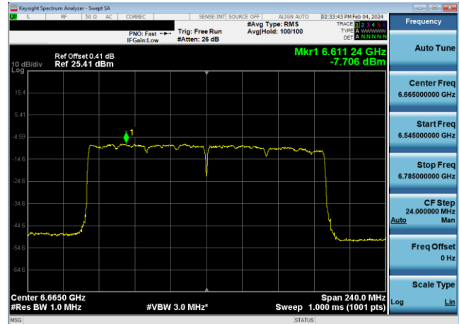
Plot 7-683. Power Spectral Density Plot SDM Diversity Antenna W7 LPI (160MHz 802.11ax (UNII Band 7) – Ch. 143, MCS11)
