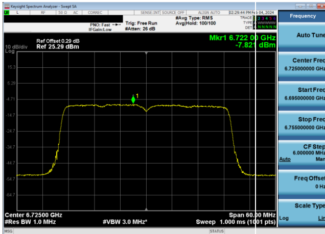
Plot 7-679. Power Spectral Density Plot SDM Diversity Antenna W7 LPI (40MHz 802.11ax (UNII Band 7) – Ch. 155, MCS11)
