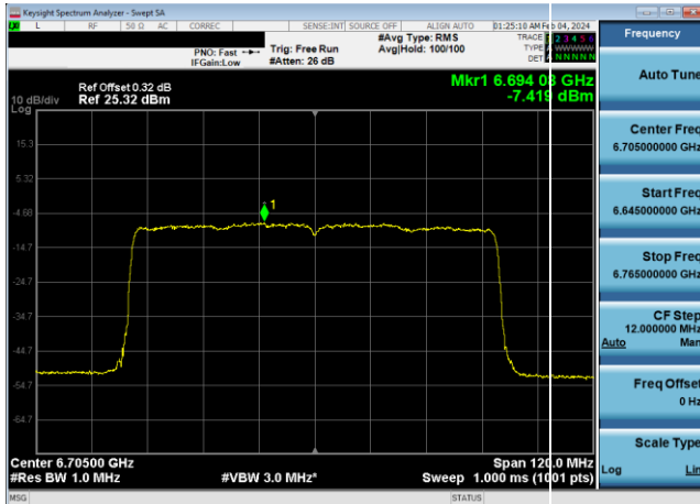
Plot 7-680. Power Spectral Density Plot SDM Diversity Antenna W8 LPI (80MHz 802.11ax (UNII Band 7) – Ch. 151, MCS11)
