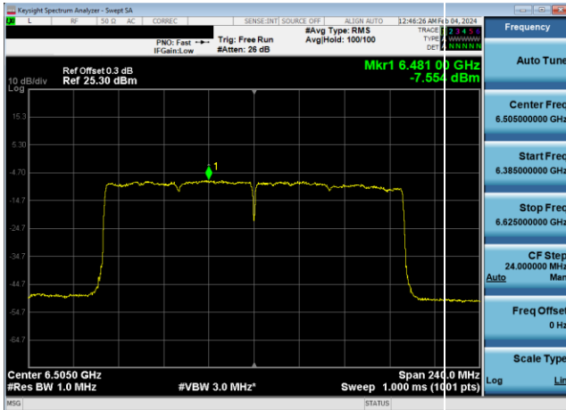
Plot 7-642. Power Spectral Density Plot SDM Diversity Antenna WF8 LPI (160MHz 802.11ax (UNII Band 6) – Ch. 111, MCS4)
