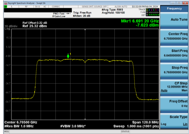
Plot 7-681. Power Spectral Density Plot SDM Diversity Antenna W7 LPI (80MHz 802.11ax (UNII Band 7) – Ch. 151, MCS11)
