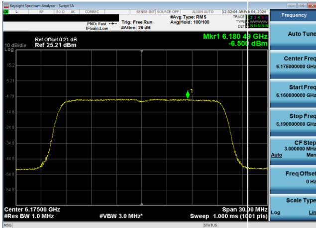
Plot 7-628. Power Spectral Density Plot SDM Diversity Antenna WF8 LPI (20MHz 802.11ax (UNII Band 5) – Ch. 45, MCS4)
