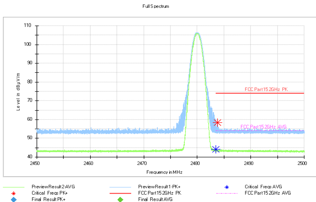
Fig.14. Frequency Band Edges: GFSK, Channel 78, 2.45 GHz - 2.50GHz
