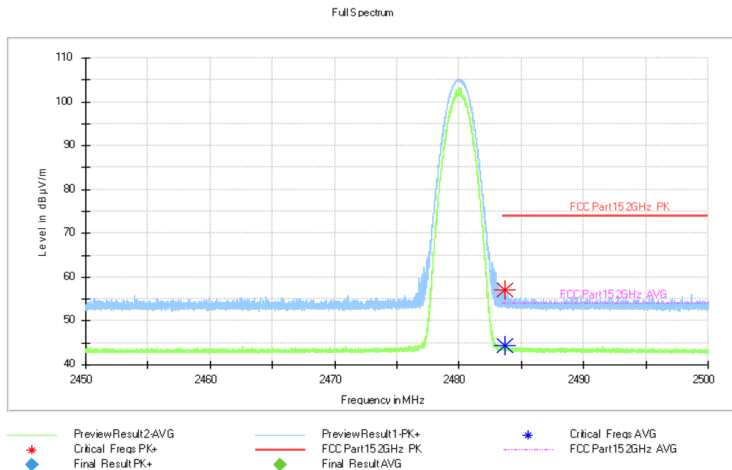
Fig.18. Frequency Band Edges: 8DPSK, Channel 78, 2.45 GHz - 2.50GHz
