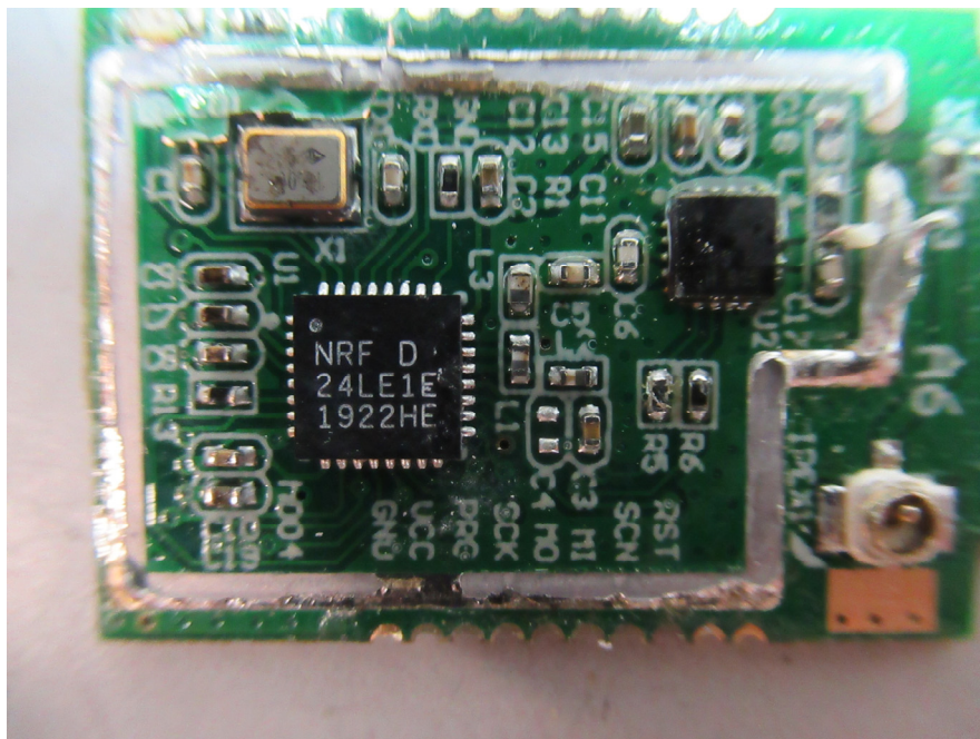
EUT – PCB Chip View (Model: HM2401A)
