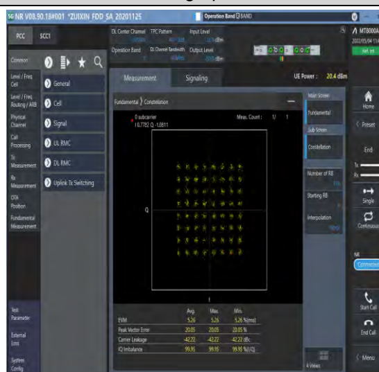
1-N7-PC3-15-40-M-8-CP-64QAM-Outer_Full-216@0-Ant1-see graph-PASS
