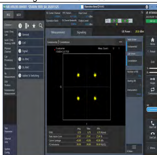
1-N7-PC3-15-40-M-6-CP-QPSK-Outer_Full-216@0-Ant1-see graph-PASS
