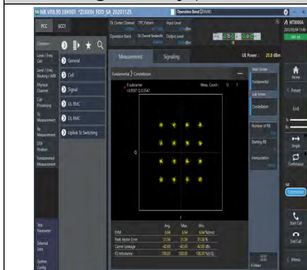
1-N7-PC3-15-40-M-7-CP-16QAM-Outer_Full-216@0-Ant1-see graph-PASS
