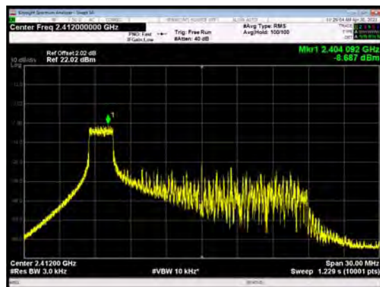
802.11ax(HE20), Channel No.: 1 26-Tones
