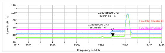
Bluetooth LE (1M) Channel 0 Peak&amp; Average
