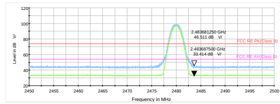
Bluetooth LE (1M) Channel 39 Peak&amp; Average
