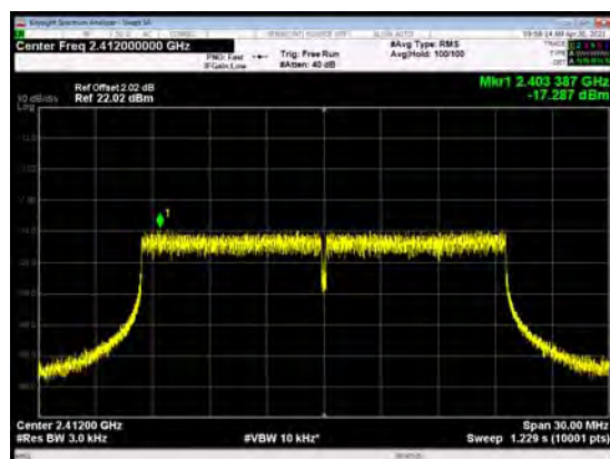
802.11ax(HE20), Channel No.: 1 242-Tones
