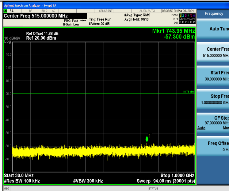
2DH5-Ant1-2441-30~1000-PASS
