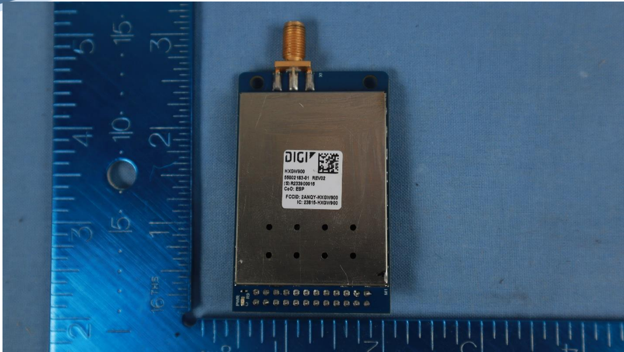
Internal Digi Radio Top Shielded
