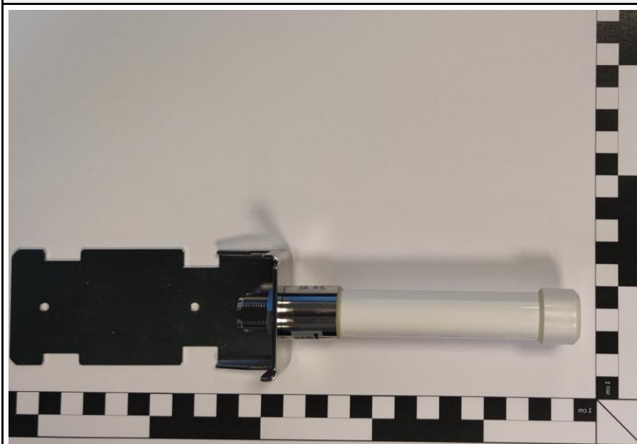
Wireless HART Antenna 1399.17.0237
