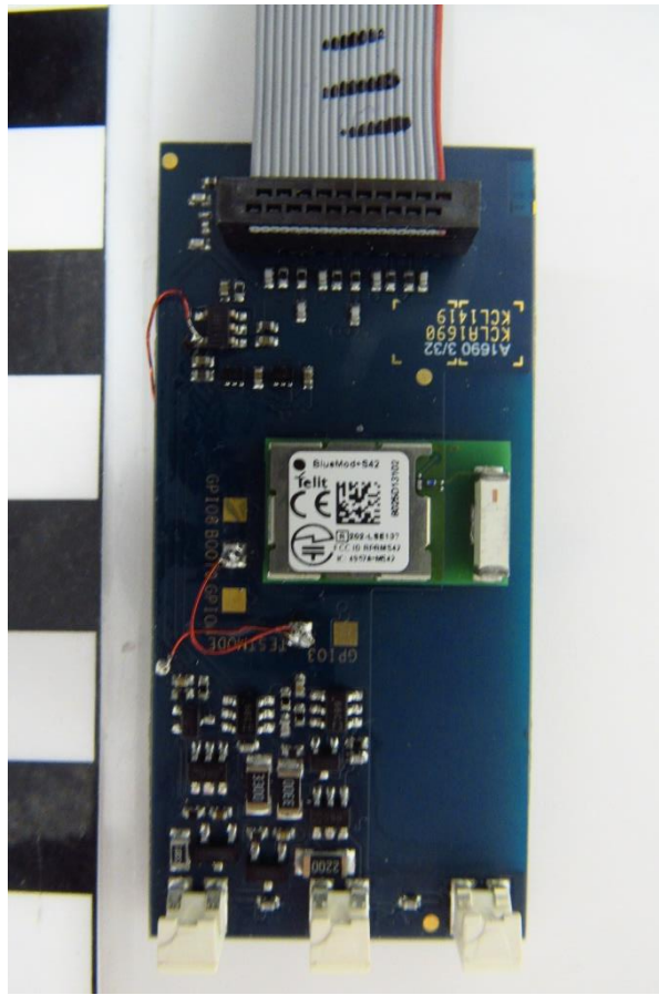
LE PCB top view
