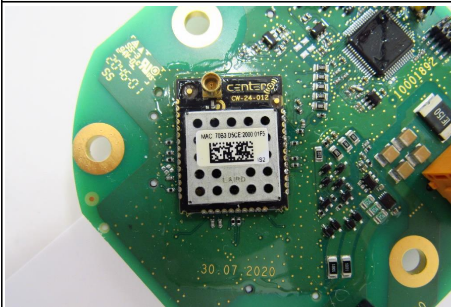
Zigbee radio
