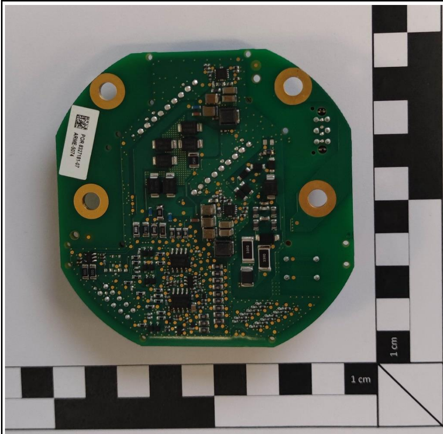
Main PCB bottom side view without casting compound
