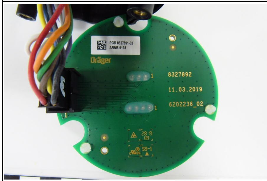
Sensor interface PCB bottom side view
