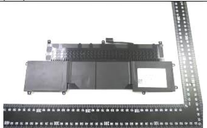
Battery (6cell)
