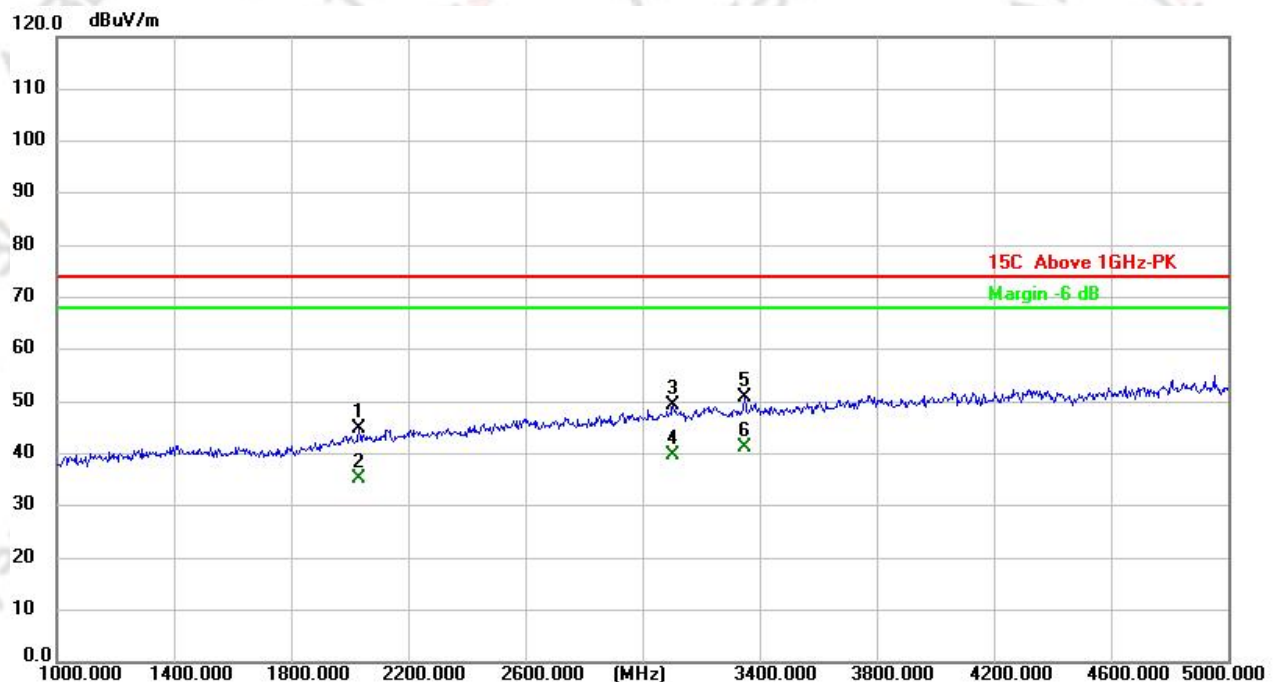
Antenna Vertical
