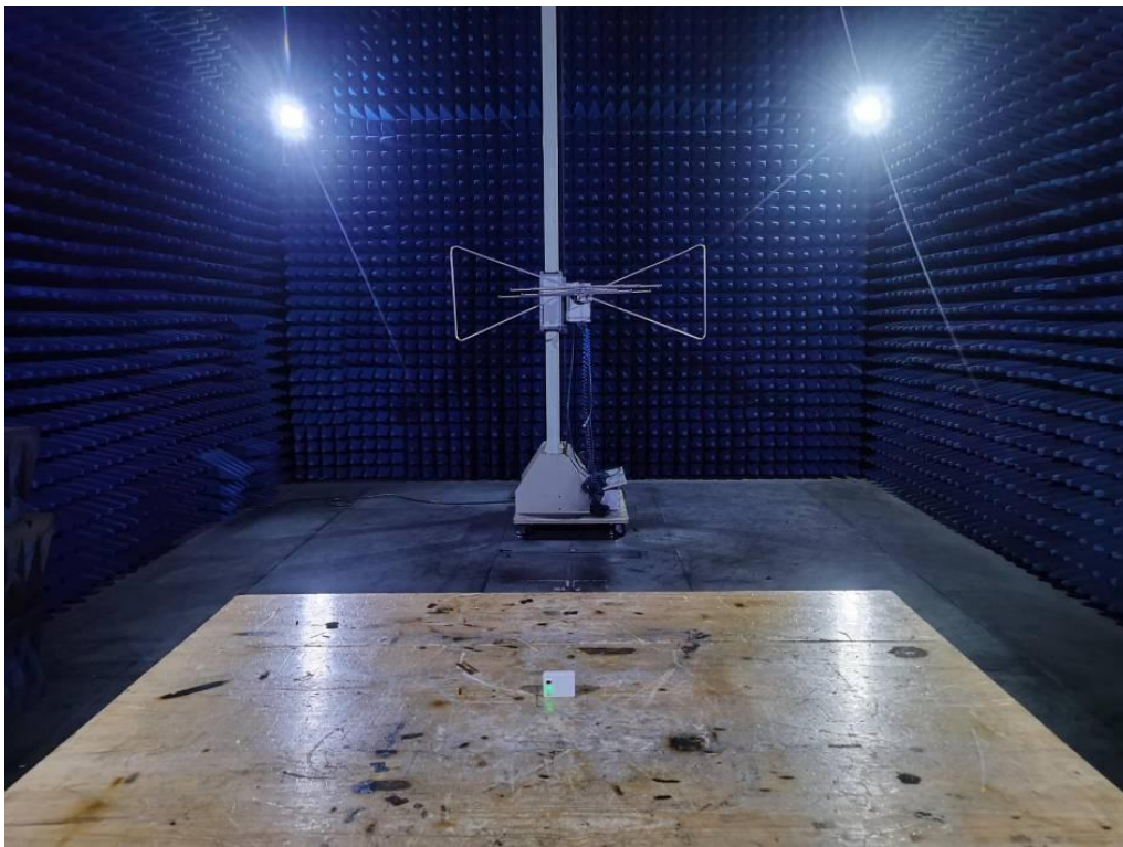
Photo of Radiated Emission Measurement (Below 1G)
