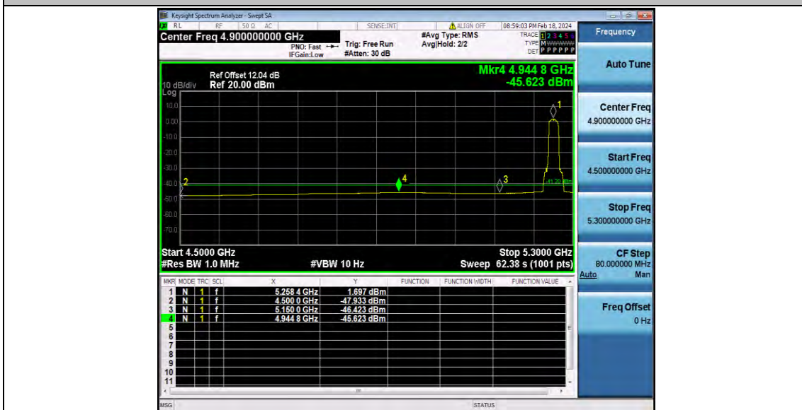
11AX20SISO_Ant1_Low_5260_Peak
