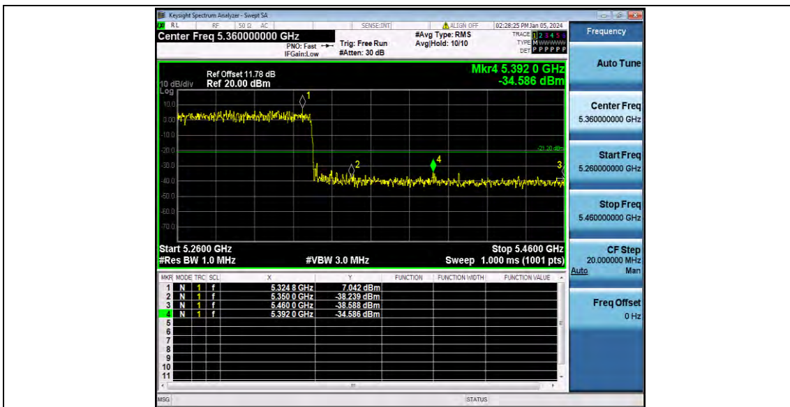
11AX20SISO_Ant1_Low_5260_AV
