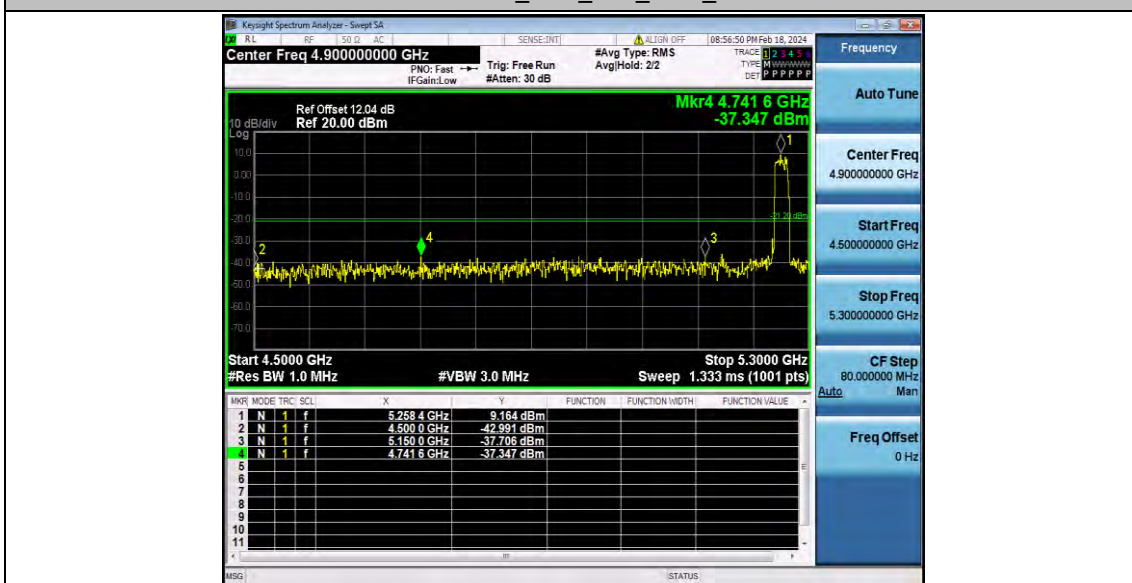
11AX20SISO_Ant1_Low_5260_Peak
