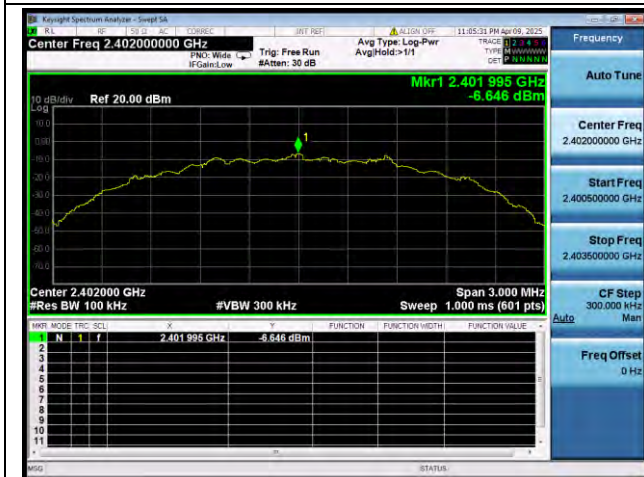
Bluetooth Low Energy 2Mbps
