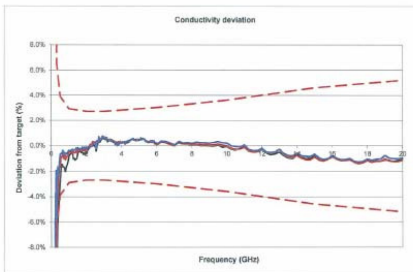
Fig. 3.2 Methanol conductivity deviation from target, 200 MHz – 20 GHz
