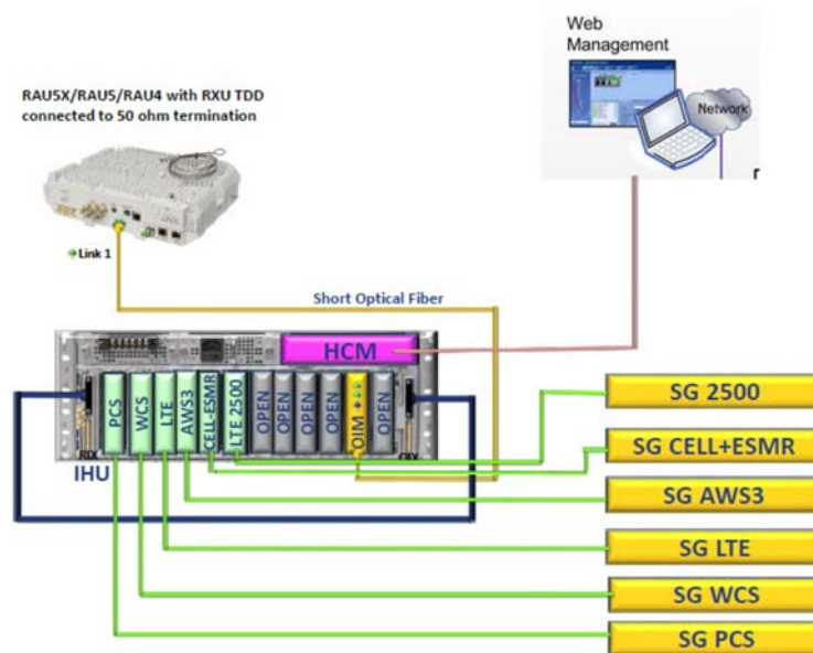
Figure 2. Radiated Test Set-Up
