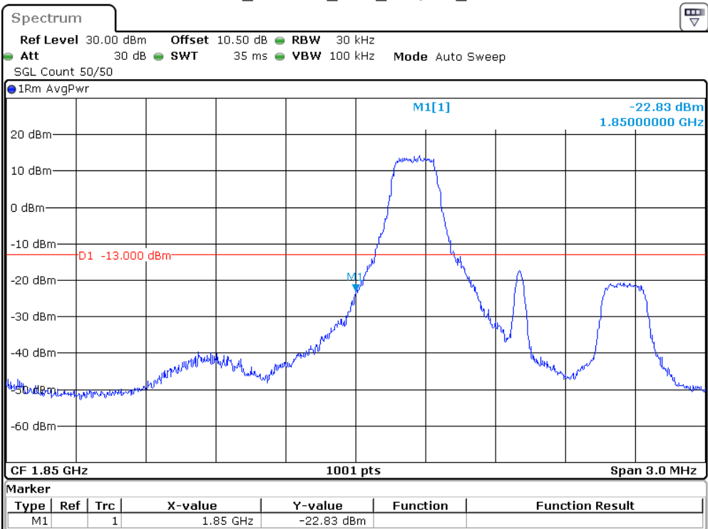
Band 2_1.4 MHz_Low_16QAM_RB1#0
