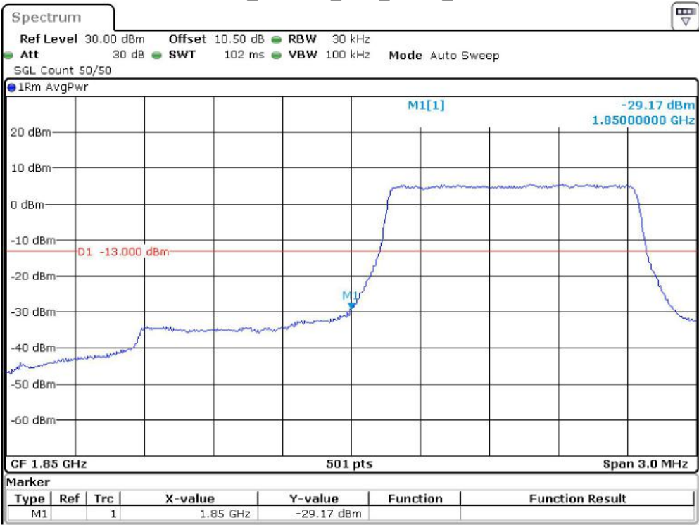
Band 2_1.4 MHz_Low_QPSK_RB6#0
