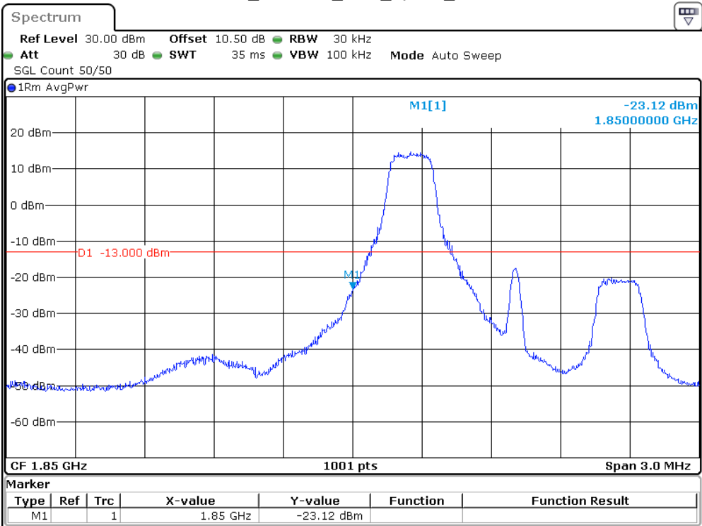
Band 2_1.4 MHz_Low_QPSK_RB1#0
