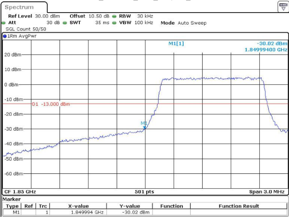
Band 2_1.4 MHz_Low_16QAM_RB6#0
