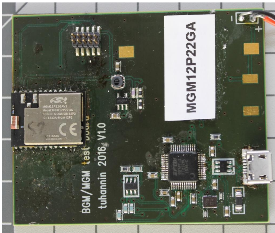
Photograph 1. EUT
