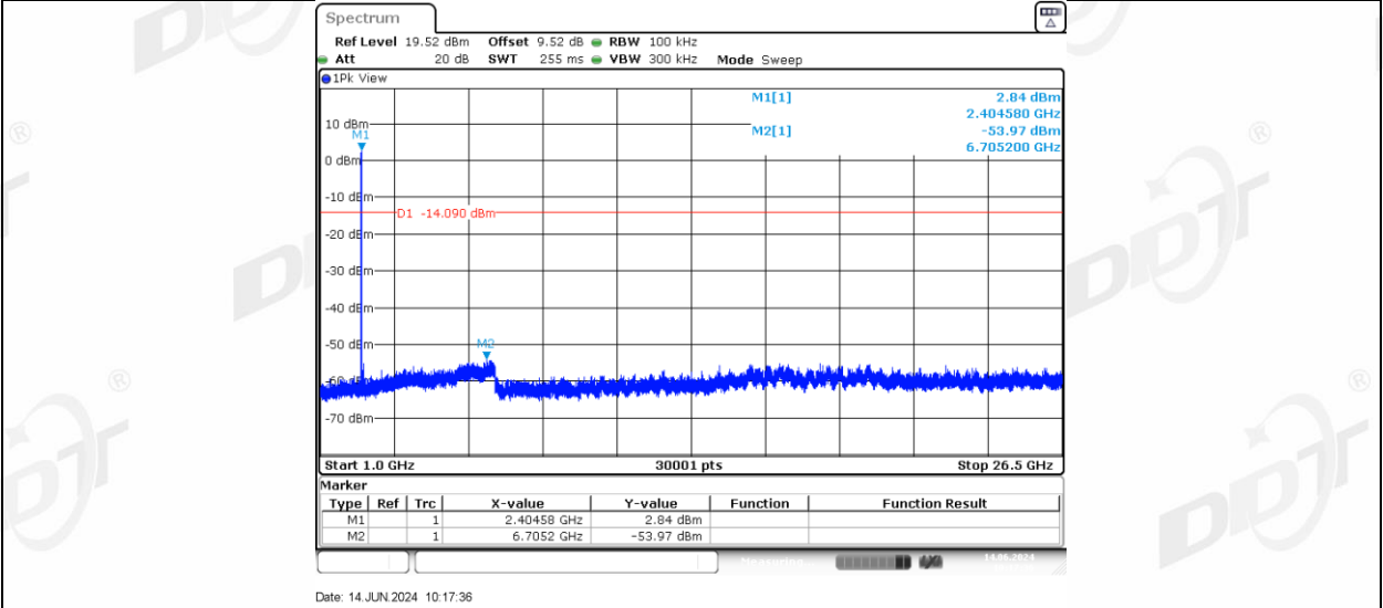
BLE_2M_Right side_2404_0~Reference
