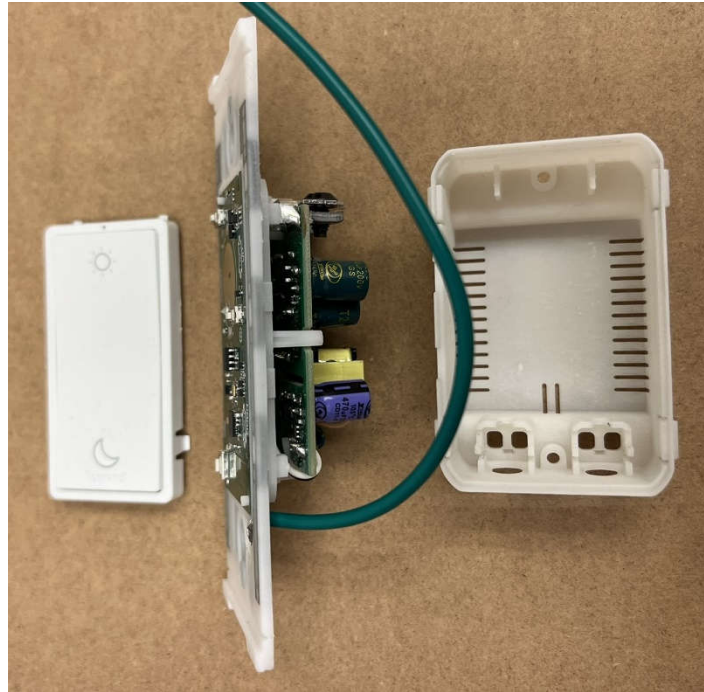
WZ3RL44 Front and Back Cover Removed
