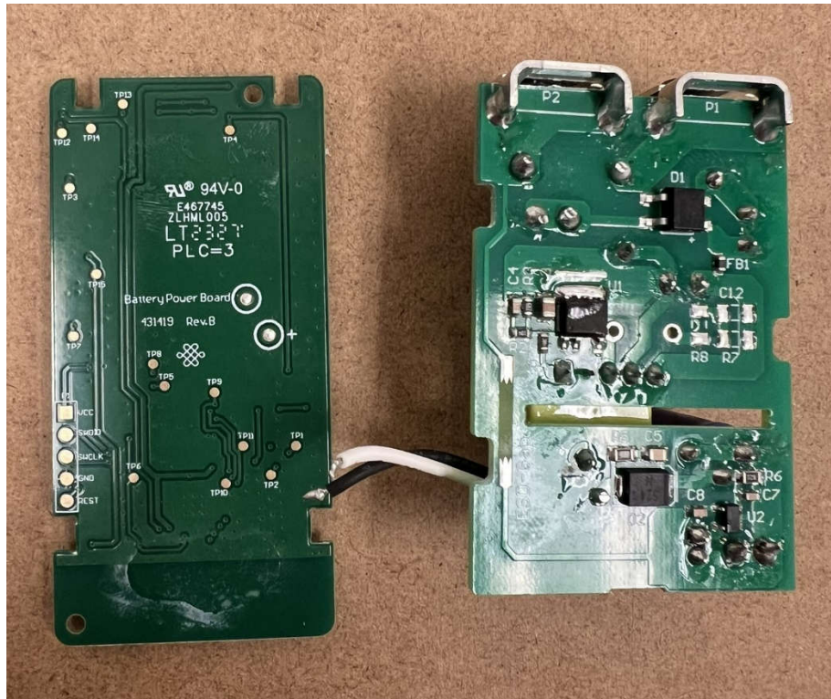
WZ3RL44 RF Board Back Side (Left) – AC Board Top Side (Right)
