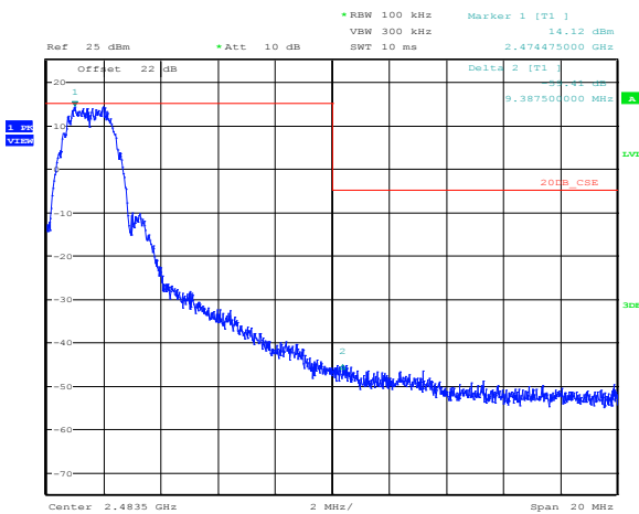
Figure 8.4-5: Conducted spurious emissions at the upper band edge, high channel
