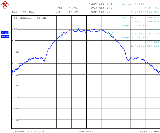
Figure 8.2-2: 6 dB bandwidth on mid channel
