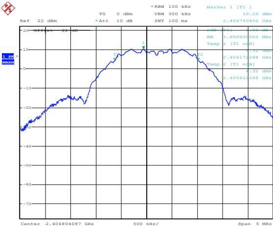
Figure 8.2-1: 6 dB bandwidth on low channel
