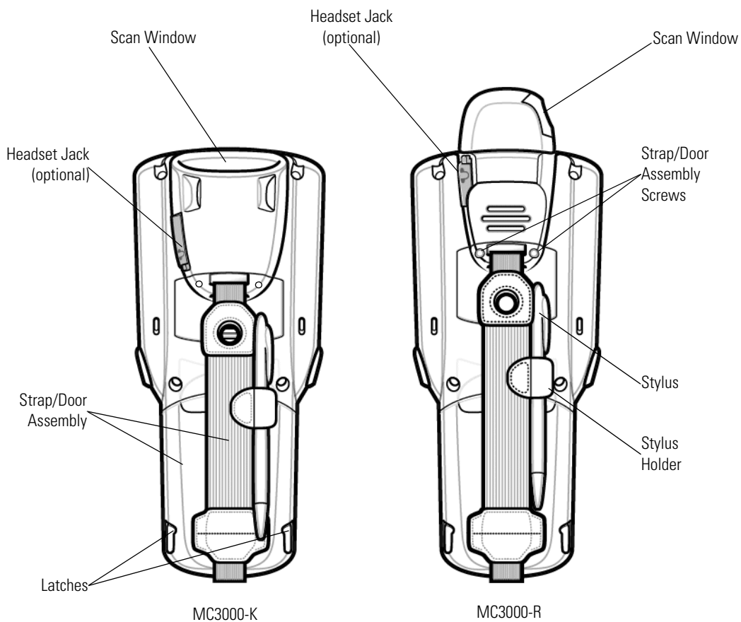
Figure 1-2. MC3000 Imager and MC3000 Laser Mobile Computers (Back View)
