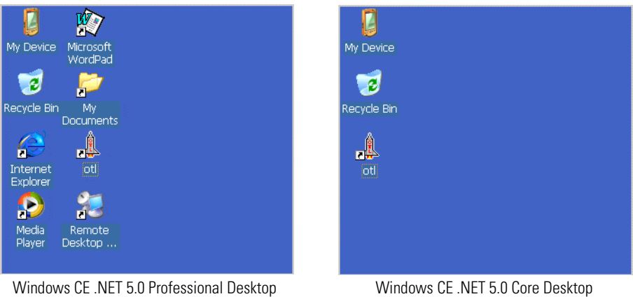
Figure 2-5. Desktop Window
