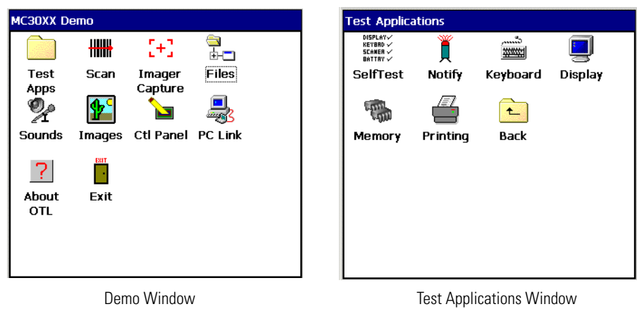
Figure 2-4. Demo Window
