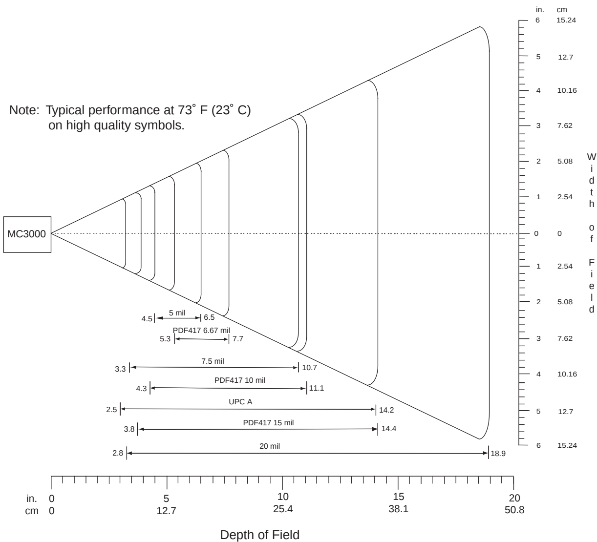
Figure 2-19. MC3000 Imager Decode Ranges
