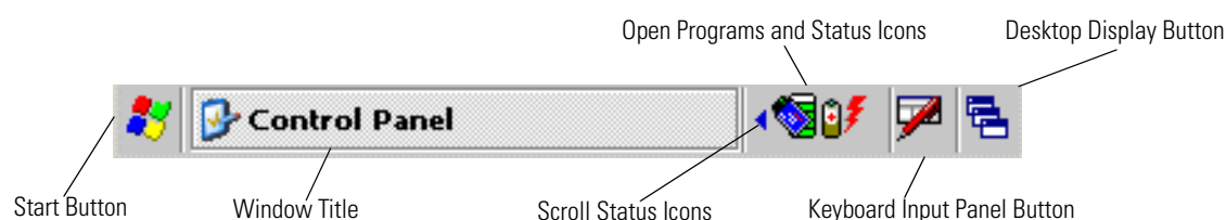
Figure 2-6. Taskbar
