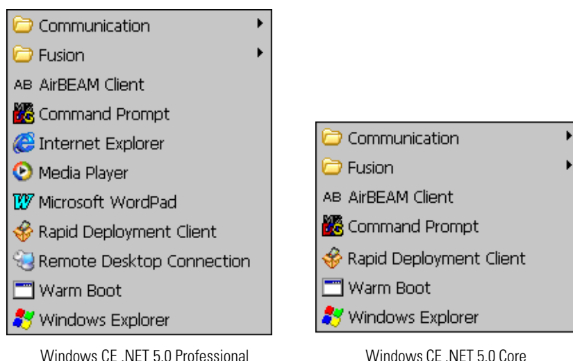
Figure 2-8. Programs Menu
