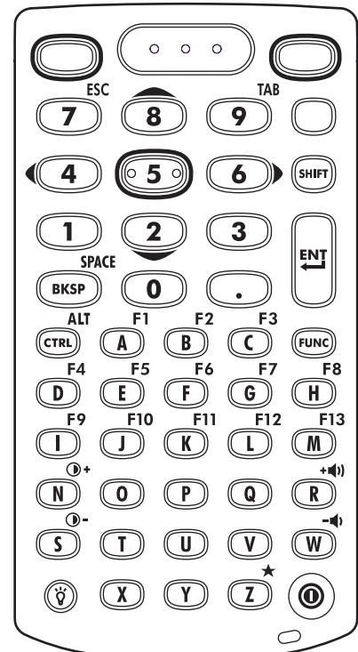
48-Key Keypad
