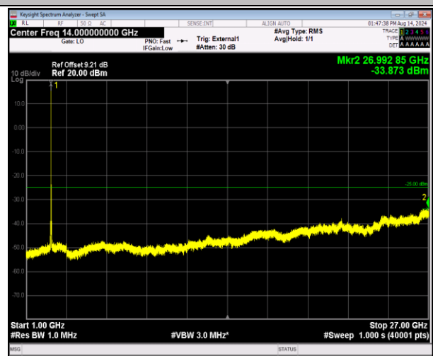
41-41-20MHz-5MHz-16QAM-16QAM-40715-40832-1RB#0- 0RB#0-1000~27000MHz-PASS
