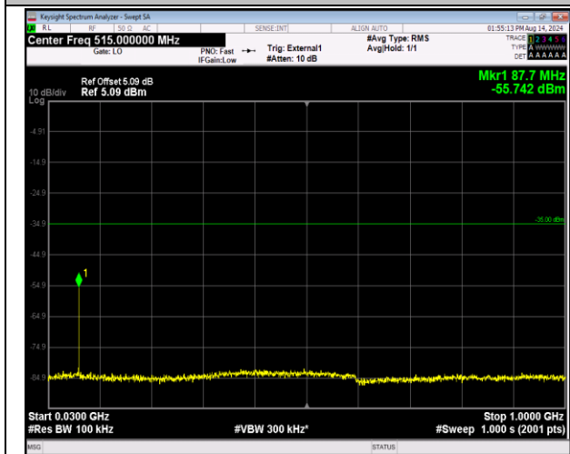
41-41-20MHz-5MHz-QPSK-QPSK-41090-41207-1RB#99-0RB#0-30~1000MHz-PASS
