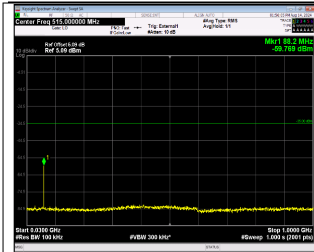
41-41-20MHz-5MHz-16QAM-16QAM-41090-41207-1RB# 99-ORB#0-30~1000MHz-PASS
