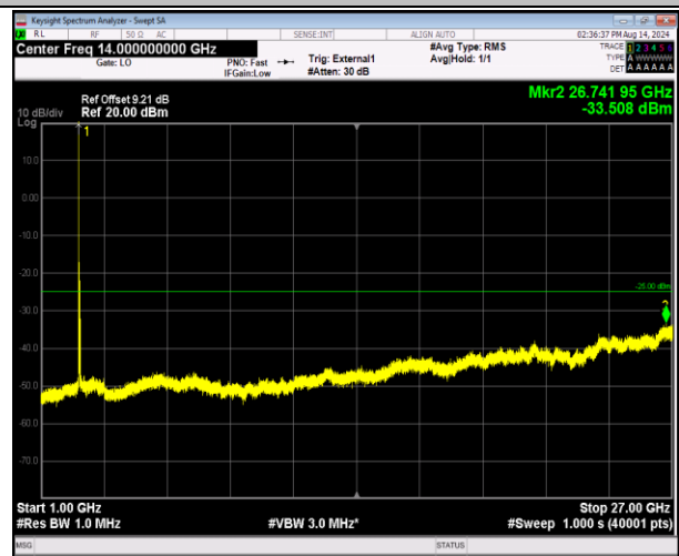
41-41-20MHz-20MHz-16QAM-16QAM-40340-40538-1RB#0 -0RB#0-1000~27000MHz-PASS
