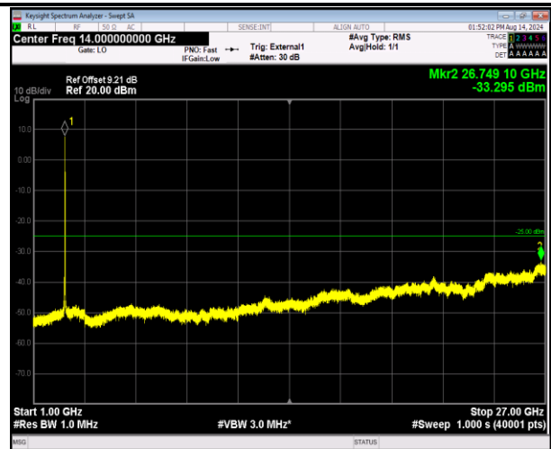
41-41-20MHz-5MHz-QPSK-QPSK-40715-40832-100RB#0- 25RB#0-1000~27000MHz-PASS
