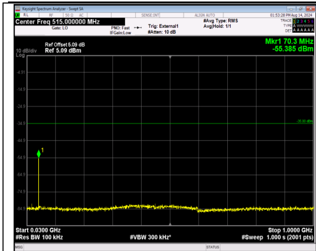
41-41-20MHz-5MHz-QPSK-QPSK-41090-41207-1RB#0-0RB#0-30~1000MHz-PASS
