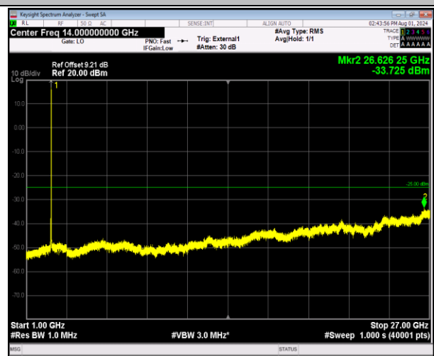
41-41-20MHz-5MHz-64QAM-64QAM-40715-40832-1RB#99 -0RB#0-1000~27000MHz-PASS
