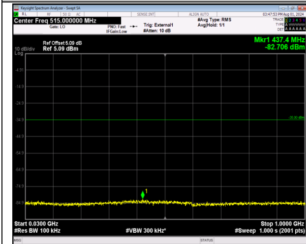
41-41-20MHz-20MHz-64QAM-64QAM-40340-40538-1RB #0-0RB#0-30~1000MHz-PASS
