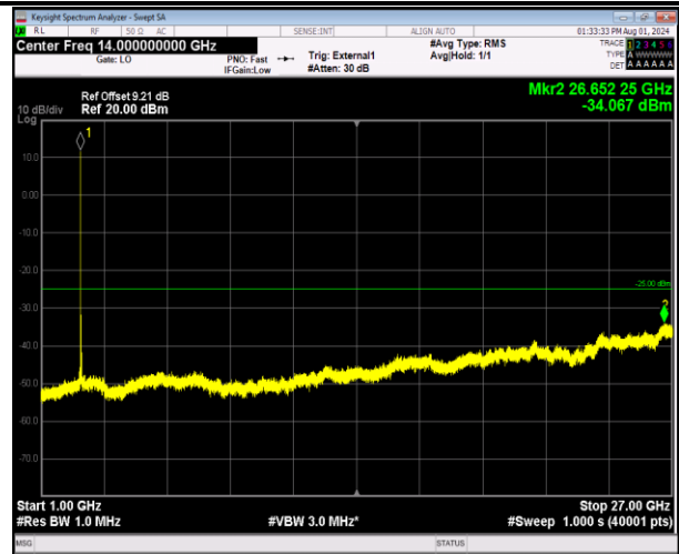
41-41-5MHz-20MHz-64QAM-64QAM-41023-41140-1RB#0- 1RB#99-1000-27000MHz-PASS
