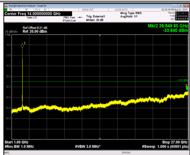
41-41-20MHz-5MHz-64QAM-64QAM-40715-40832-100RB# 0-25RB#0-1000~27000MHz-PASS
