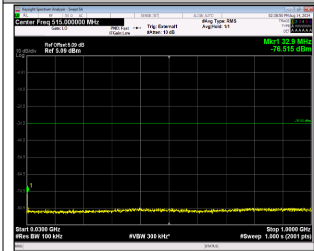
41-41-20MHz-20MHz-QPSK-QPSK-40340-40538-1RB#0 -1RB#99-30~1000MHz-PASS
