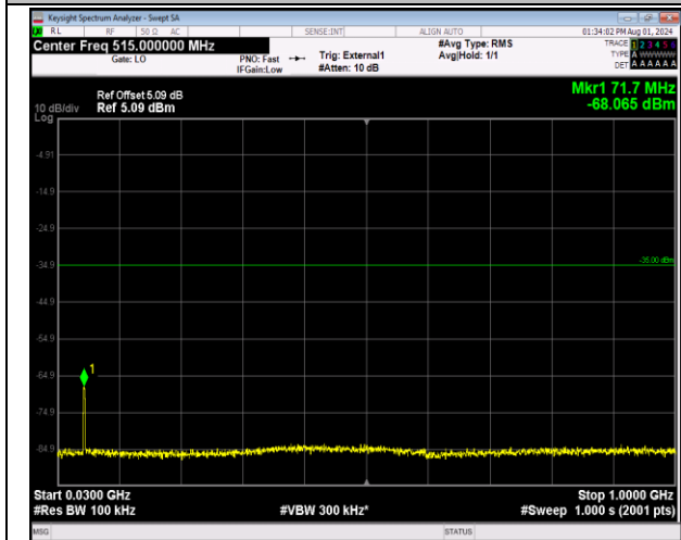
41-41-5MHz-20MHz-64QAM-64QAM-41023-41140-25RB #0-100RB#0-30-1000MHz-PASS
