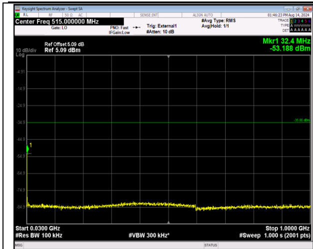
41-41-20MHz-5MHz-QPSK-QPSK-40715-40832-1RB#0-0RB#0-30~1000MHz-PASS
