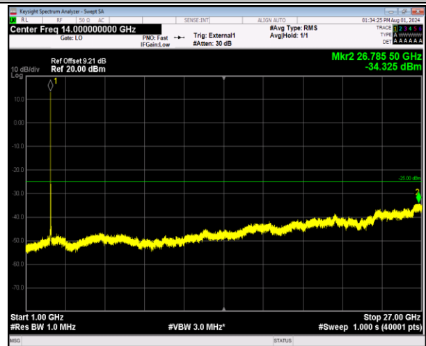
41-41-5MHz-20MHz-64QAM-64QAM-41023-41140-25RB#0 -100RB#0-1000-27000MHz-PASS
