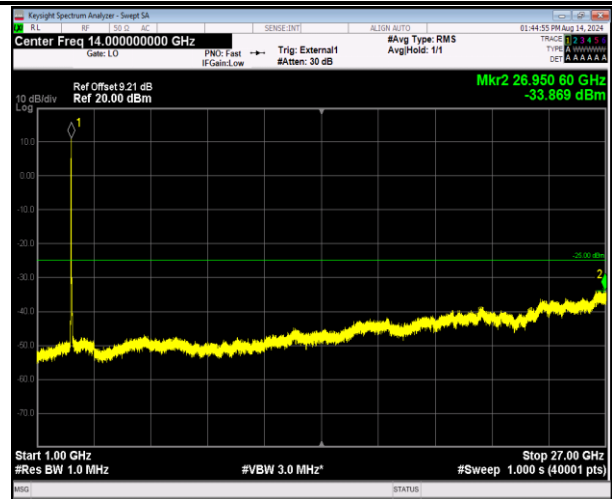
41-41-20MHz-5MHz-QPSK-QPSK-40340-40457-100RB#0- 25RB#0-1000-27000MHz-PASS
