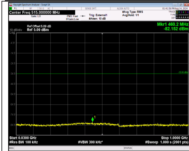
41-41-20MHz-5MHz-16QAM-16QAM-40340-40457-1RB# 99-ORB#0-30~1000MHz-PASS
