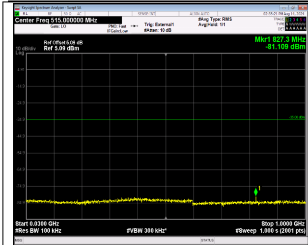
41-41-20MHz-20MHz-QPSK-QPSK-40340-40538-1RB#0 -ORB#0-30~1000MHz-PASS
