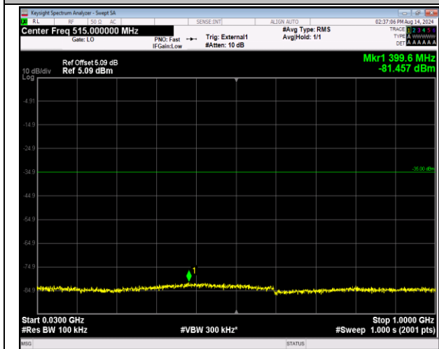
41-41-20MHz-20MHz-QPSK-QPSK-40340-40538-1RB#9 9-ORB#0-30~1000MHz-PASS
