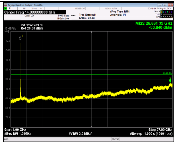
41-41-20MHz-5MHz-64QAM-64QAM-40340-40457-1RB#0- 1RB#24-1000~27000MHz-PASS
