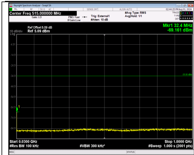
41-41-20MHz-5MHz-64QAM-64QAM-40715-40832-1RB# 0-1RB#24-30~1000MHz-PASS
