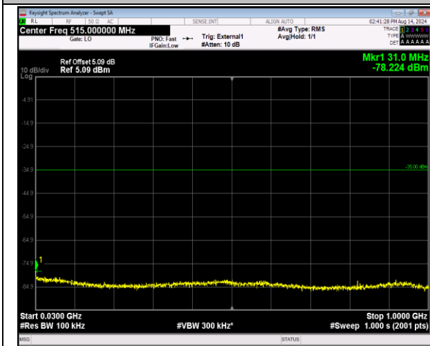
41-41-20MHz-20MHz-16QAM-16QAM-40340-40538-100RB RB#0-100RB#0-30~1000MHz-PASS
