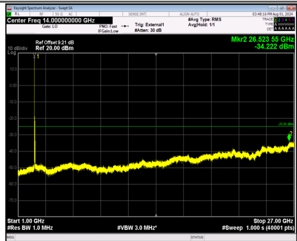
41-41-20MHz-20MHz-64QAM-64QAM-40340-40538-1RB#0 -0RB#0-1000~27000MHz-PASS
