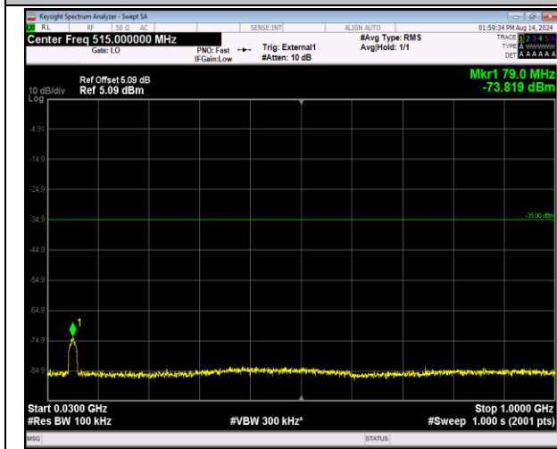
41-41-20MHz-5MHz-16QAM-16QAM-41090-41207-100R B#0-25RB#0-30~1000MHz-PASS
