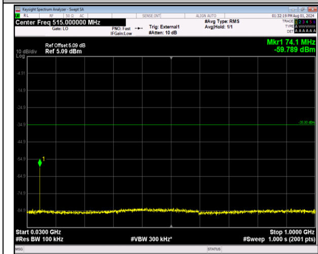
41-41-5MHz-20MHz-64QAM-64QAM-41023-41140-1RB# 24-0RB#0-30-1000MHz-PASS
