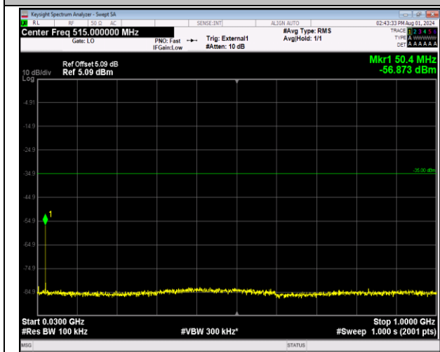
41-41-20MHz-5MHz-64QAM-64QAM-40715-40832-1RB# 99-0RB#0-30~1000MHz-PASS
