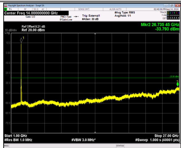
41-41-20MHz-20MHz-16QAM-16QAM-40340-40538-1RB#0 -1RB#99-1000~27000MHz-PASS
