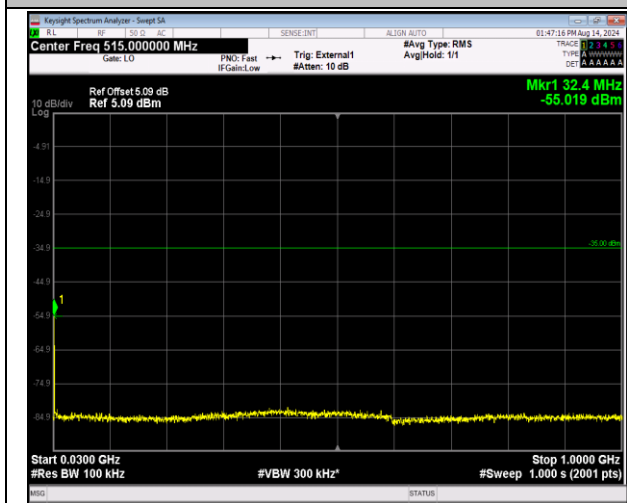
41-41-20MHz-5MHz-16QAM-16QAM-40715-40832-1RB# 0-0RB#0-30~1000MHz-PASS
