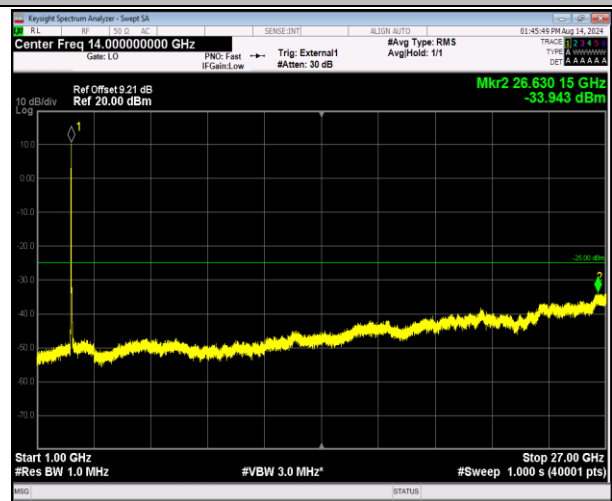
41-41-20MHz-5MHz-16QAM-16QAM-40340-40457-100RB# 0-25RB#0-1000~27000MHz-PASS
