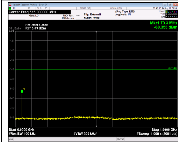
41-41-20MHz-5MHz-64QAM-64QAM-41090-41207-1RB# 0-ORB#0-30~1000MHz-PASS
