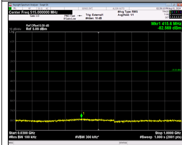
41-41-20MHz-5MHz-64QAM-64QAM-40340-40457-1RB# 0-ORB#0-30~1000MHz-PASS
