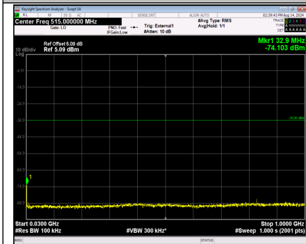
41-41-20MHz-20MHz-16QAM-16QAM-40340-40538-1RB #0-1RB#99-30~1000MHz-PASS
