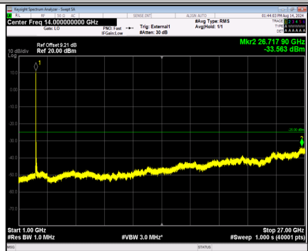
41-41-20MHz-5MHz-16QAM-16QAM-40340-40457-1RB#0- 1RB#24-1000-27000MHz-PASS
