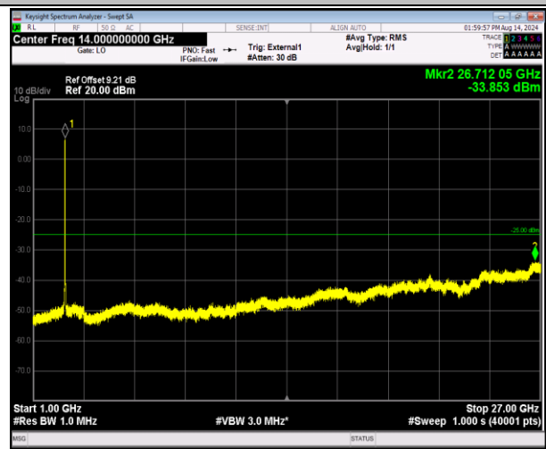
41-41-20MHz-5MHz-16QAM-16QAM-41090-41207-100RB# 0-25RB#0-1000~27000MHz-PASS
