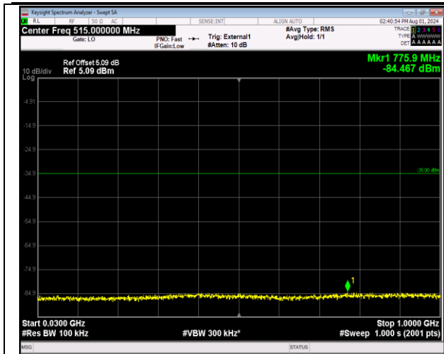
41-41-20MHz-5MHz-64QAM-64QAM-40340-40457-1RB# 0-1RB#24-30~1000MHz-PASS
