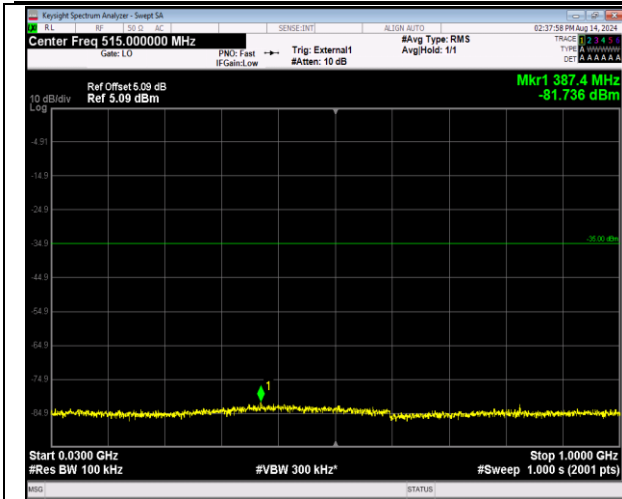
41-41-20MHz-20MHz-16QAM-16QAM-40340-40538-1RB #99-0RB#0-30~1000MHz-PASS
