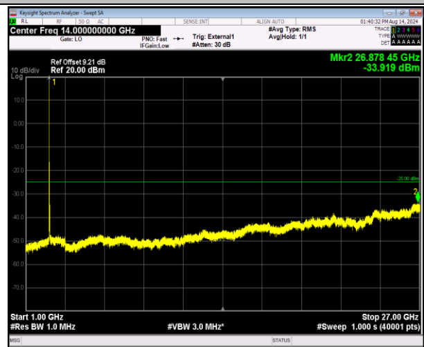
41-41-20MHz-5MHz-16QAM-16QAM-40340-40457-1RB#0- 0RB#0-1000-27000MHz-PASS
