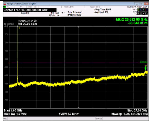
41-41-20MHz-20MHz-16QAM-16QAM-40340-40538-1RB#9 9-0RB#0-1000~27000MHz-PASS
