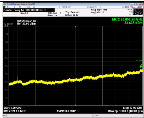
41-41-20MHz-5MHz-16QAM-16QAM-41090-41207-1RB#99 -ORB#0-1000~27000MHz-PASS
