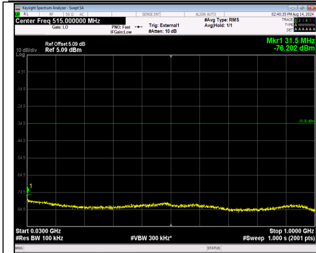
41-41-20MHz-20MHz-QPSK-QPSK-40340-40538-100RB #0-100RB#0-30~1000MHz-PASS
