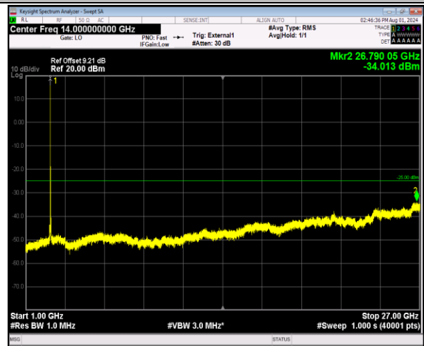
41-41-20MHz-5MHz-64QAM-64QAM-41090-41207-1RB#0- ORB#0-1000~27000MHz-PASS
