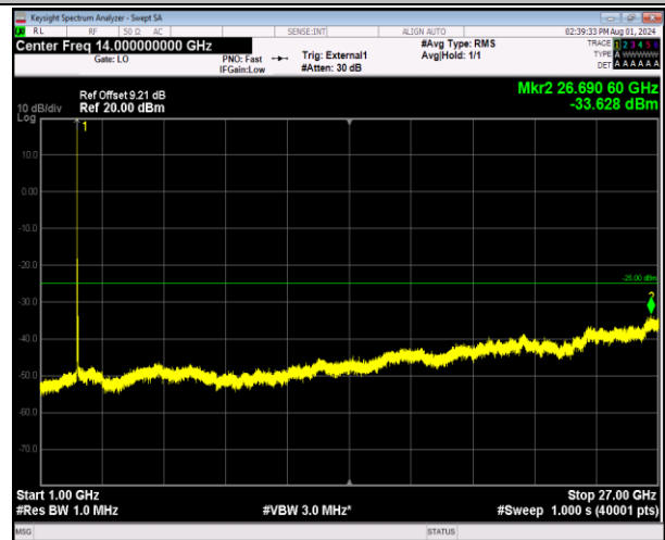
41-41-20MHz-5MHz-64QAM-64QAM-40340-40457-1RB#0- ORB#0-1000~27000MHz-PASS
