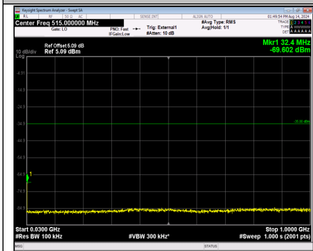
41-41-20MHz-5MHz-QPSK-QPSK-40715-40832-1RB#0-01RB#24-30~1000MHz-PASS
