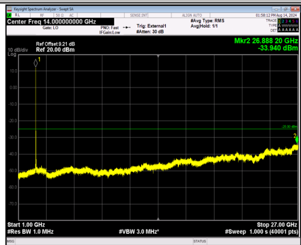
41-41-20MHz-5MHz-16QAM-16QAM-41090-41207-1RB#0- 1RB#24-1000~27000MHz-PASS
