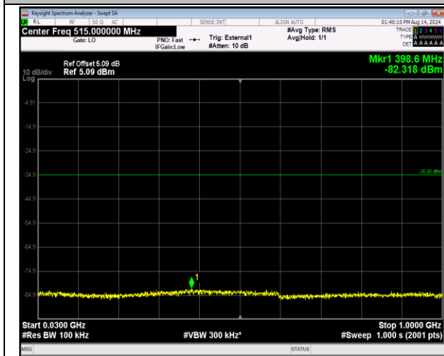
41-41-20MHz-5MHz-16QAM-16QAM-40340-40457-1RB# 0-0RB#0-30-1000MHz-PASS
