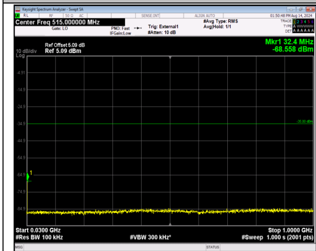
41-41-20MHz-5MHz-16QAM-16QAM-40715-40832-1RB# 0-1RB#24-30~1000MHz-PASS
