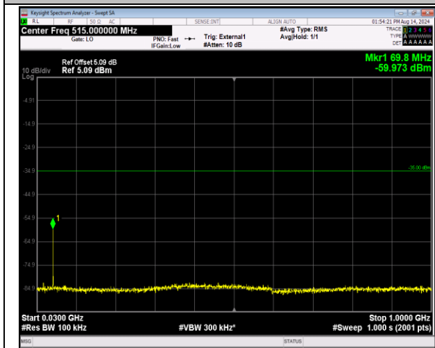
41-41-20MHz-5MHz-16QAM-16QAM-41090-41207-1RB# 0-0RB#0-30~1000MHz-PASS
