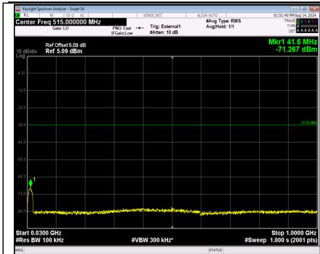
41-41-20MHz-5MHz-QPSK-QPSK-40715-40832-100RB# 0-25RB#0-30~1000MHz-PASS
