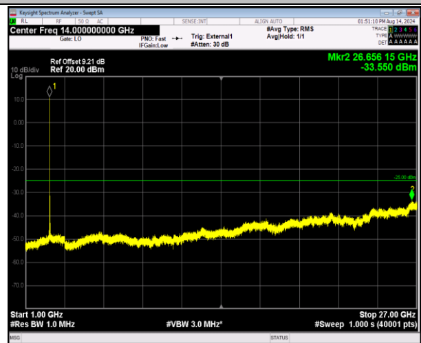
41-41-20MHz-5MHz-16QAM-16QAM-40715-40832-1RB#0- 1RB#24-1000~27000MHz-PASS
