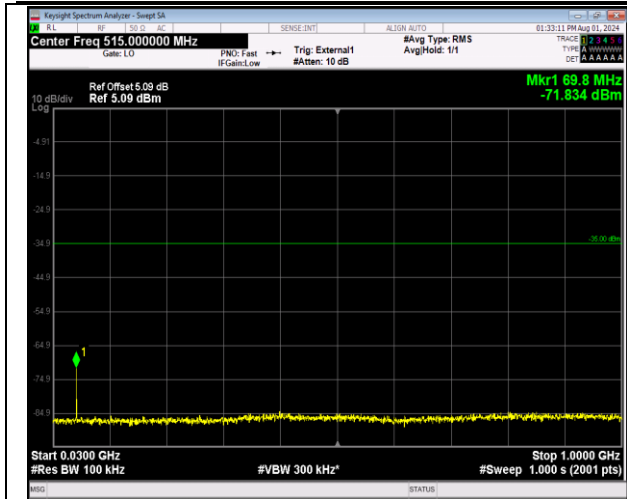
41-41-5MHz-20MHz-64QAM-64QAM-41023-41140-1RB# 0-1RB#99-30-1000MHz-PASS
