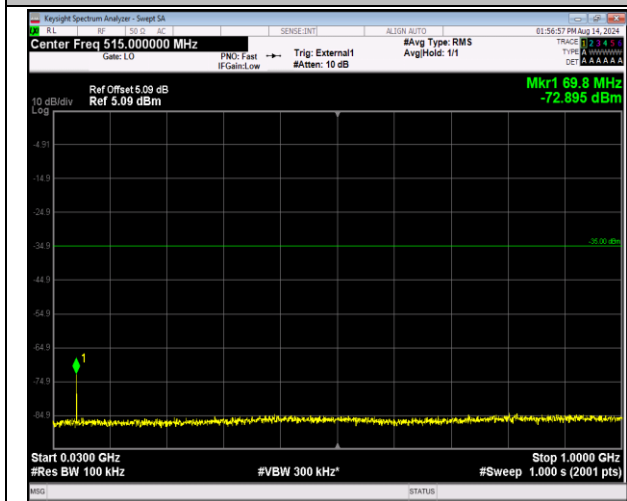
41-41-20MHz-5MHz-QPSK-QPSK-41090-41207-1RB#0-01RB#24-30~1000MHz-PASS
