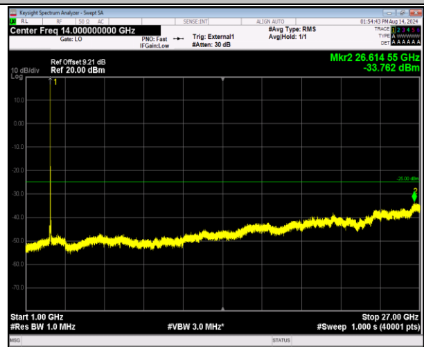
41-41-20MHz-5MHz-16QAM-16QAM-41090-41207-1RB#0- 0RB#0-1000~27000MHz-PASS
