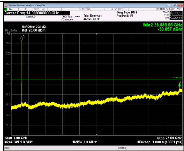
41-41-20MHz-5MHz-64QAM-64QAM-40715-40832-1RB#0- 1RB#24-1000~27000MHz-PASS
