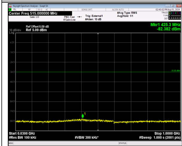
41-41-20MHz-5MHz-64QAM-64QAM-40340-40457-1RB# 99-0RB#0-30~1000MHz-PASS
