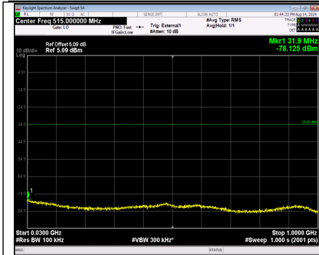
41-41-20MHz-5MHz-QPSK-QPSK-40340-40457-100RB# 0-25RB#0-30-1000MHz-PASS
