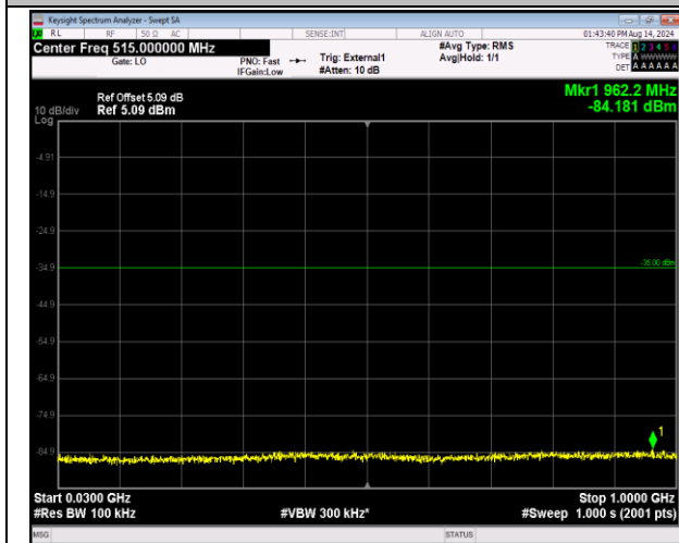
41-41-20MHz-5MHz-16QAM-16QAM-40340-40457-1RB# 0-1RB#24-30-1000MHz-PASS
