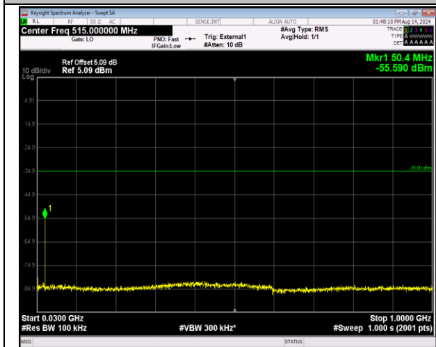
41-41-20MHz-5MHz-QPSK-QPSK-40715-40832-1RB#99-0RB#0-30~1000MHz-PASS
