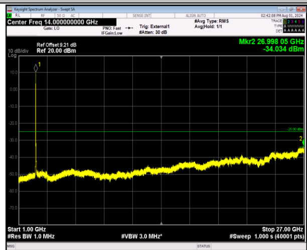
41-41-20MHz-5MHz-64QAM-64QAM-40340-40457-100RB# 0-25RB#0-1000~27000MHz-PASS
