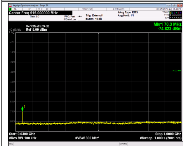
41-41-20MHz-5MHz-16QAM-16QAM-41090-41207-1RB# 0-1RB#24-30~1000MHz-PASS
