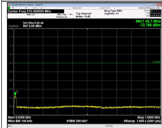
41-41-20MHz-5MHz-64QAM-64QAM-40715-40832-100R B#0-25RB#0-30~1000MHz-PASS
