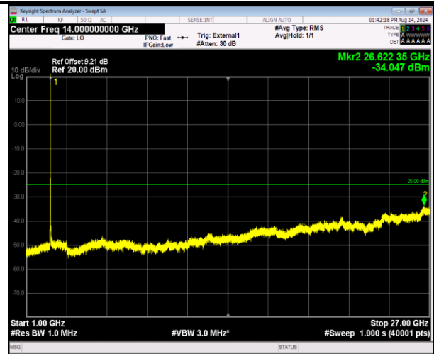
41-41-20MHz-5MHz-16QAM-16QAM-40340-40457-1RB#99 -ORB#0-1000~27000MHz-PASS
