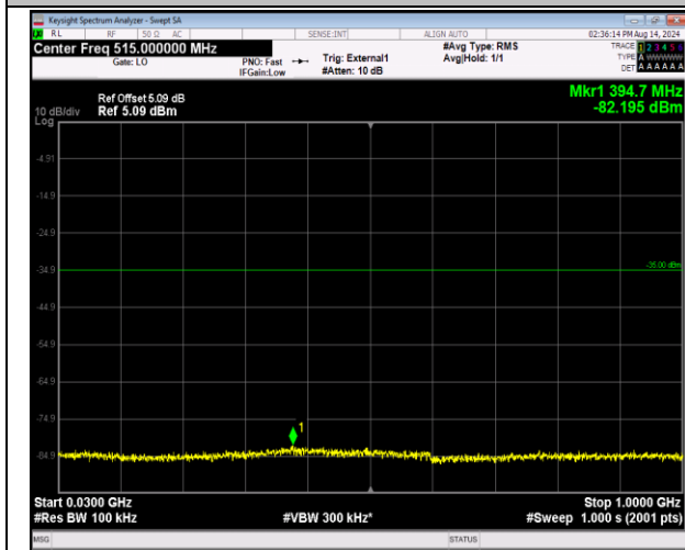
41-41-20MHz-20MHz-16QAM-16QAM-40340-40538-1RB #0-0RB#0-30~1000MHz-PASS
