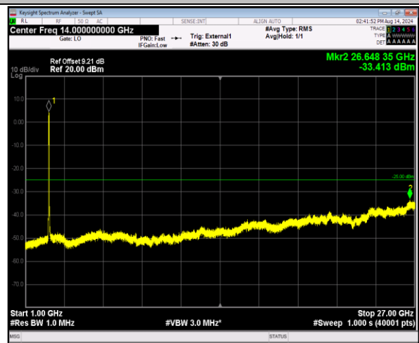
41-41-20MHz-20MHz-16QAM-16QAM-40340-40538-100RB #0-100RB#0-1000~27000MHz-PASS
