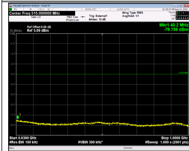
41-41-20MHz-5MHz-16QAM-16QAM-40340-40457-100R B#0-25RB#0-30~1000MHz-PASS
