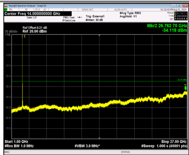
41-41-5MHz-20MHz-64QAM-64QAM-41023-41140-1RB#24 -0RB#0-1000-27000MHz-PASS
