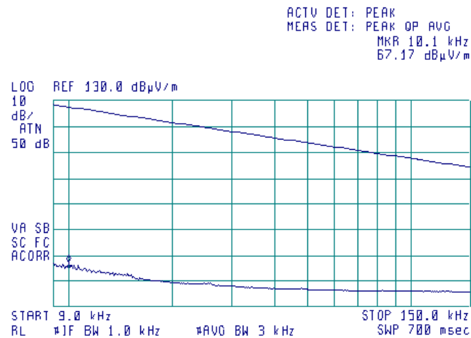
Plot 7.3.2 Radiated emission measurements from 9 to 150 kHz at high frequency
