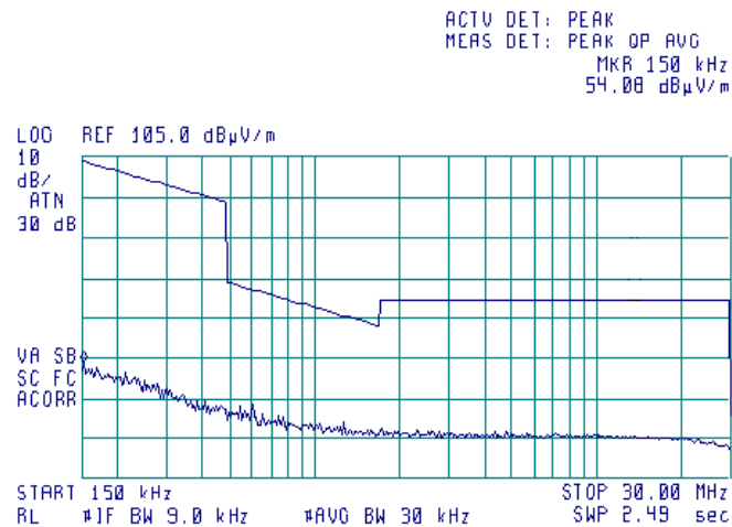
Plot 7.3.4 Radiated emission measurements from 0.15 to 30 MHz at high frequency
