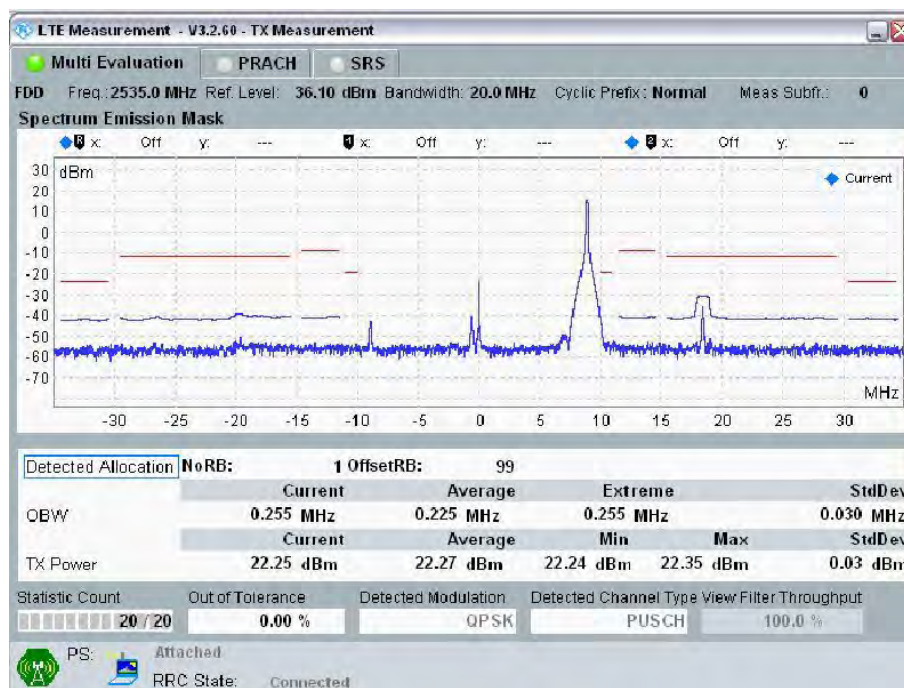
20MHz Band Width: Ch 21100, RB Size=1; RB Offset = 99
