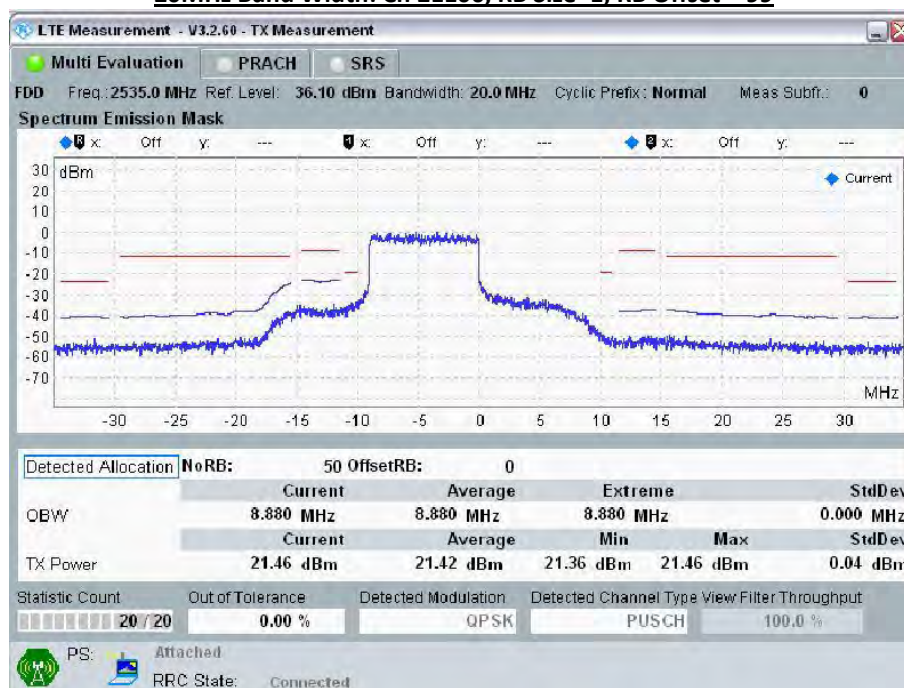
20MHz Band Width: Ch 21100, RB Size=50; RB Offset = 0
