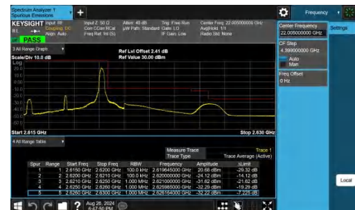
Band38-5MHz-QPSK-38225-1RB#24-PASS
