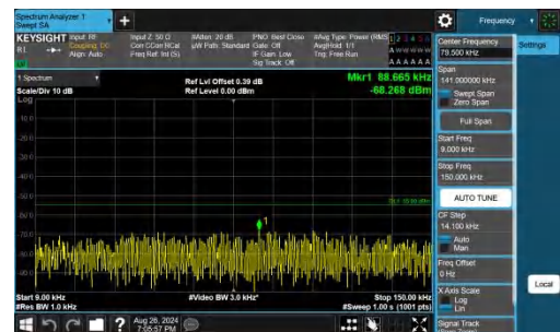
Band38-10MHz-QPSK-38000-1RB#49-0.009~0.15-PASS
