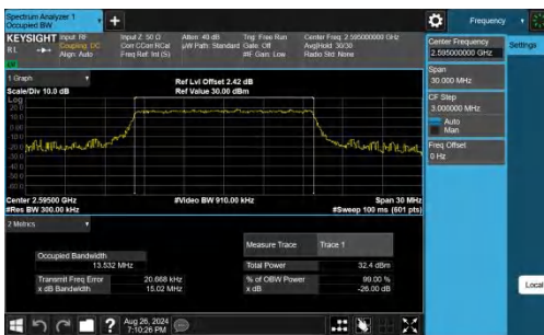
Band38-15MHz-QPSK-38000-75RB#0-PASS
