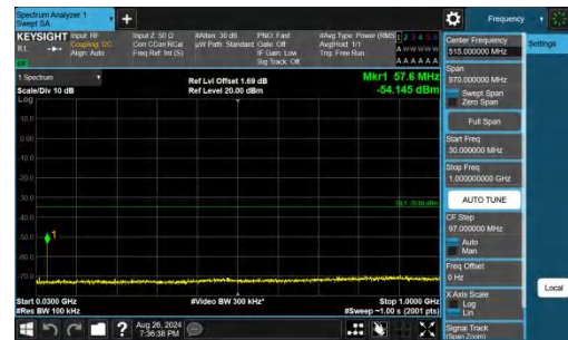
Band38-20MHz-QPSK-38150-1RB#99-30~1000-PASS
