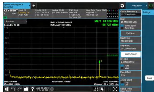
Band38-20MHz-QPSK-38000-1RB#0-0.15~30-PASS
