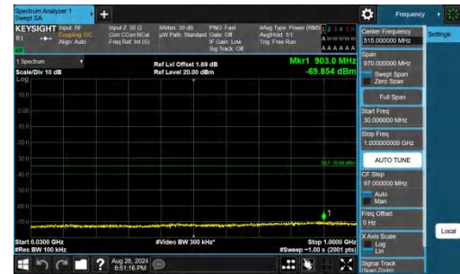
Band38-5MHz-QPSK-38000-1RB#24-30~1000-PASS
