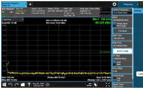
Band38-5MHz-QPSK-38225-1RB#24-0.15~30-PASS
