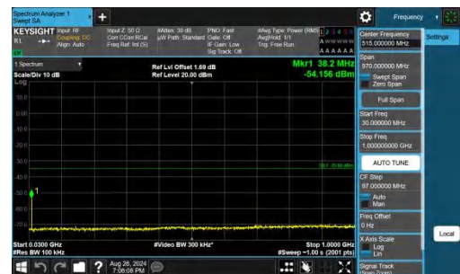
Band38-10MHz-QPSK-38000-1RB#49-30~1000-PASS
