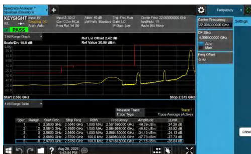
Band38-5MHz-QPSK-37775-1RB#24-PASS
