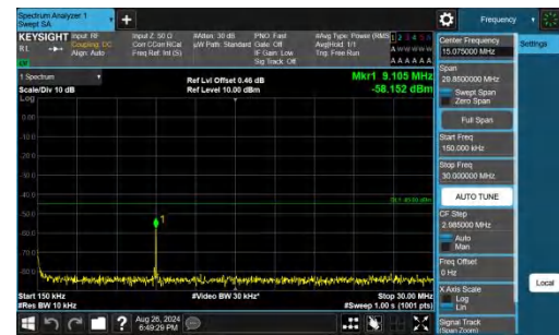
Band38-5MHz-QPSK-37775-1RB#0-0.15~30-PASS
