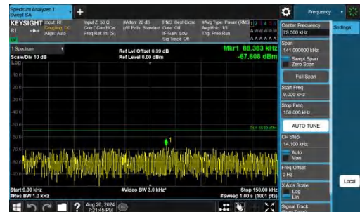
Band38-15MHz-QPSK-38175-1RB#74-0.009~0.15-PASS
