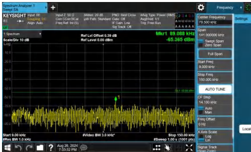
Band38-20MHz-QPSK-37850-1RB#0-0.009~0.15-PASS
