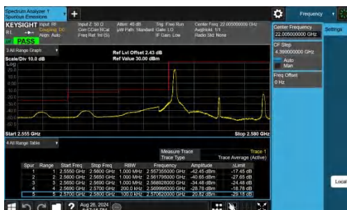
Band38-10MHz-QPSK-37800-1RB#0-PASS
