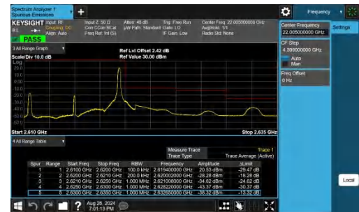
Band38-10MHz-QPSK-38200-1RB#49-PASS
