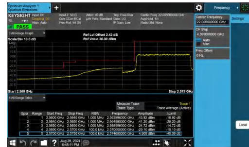
Band38-5MHz-QPSK-37775-25RB#0-PASS
