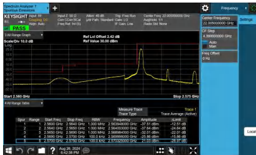
Band38-5MHz-QPSK-37775-1RB#0-PASS
