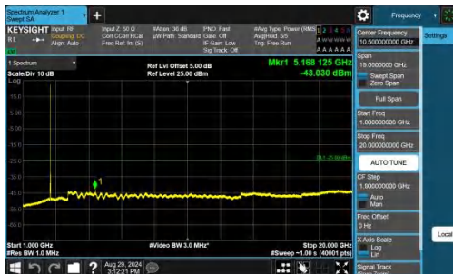
Band38-15MHz-QPSK-37825-1RB#74-1000~20000-PASS
