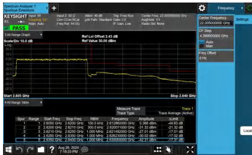
Band38-15MHz-QPSK-38175-75RB#0-PASS
