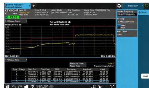
Band38-10MHz-QPSK-37800-50RB#0-PASS
