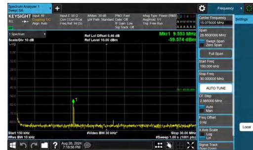
Band38-15MHz-QPSK-37825-1RB#0-0.15~30-PASS
