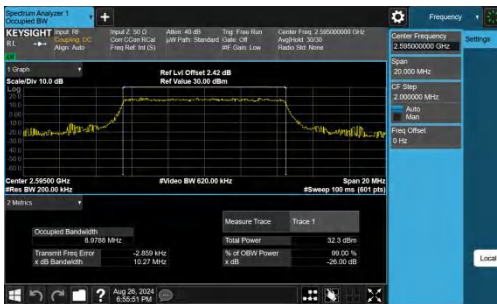
Band38-10MHz-QPSK-38000-50RB#0-PASS
