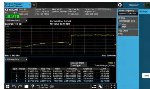
Band38-20MHz-QPSK-37850-100RB#0-PASS
