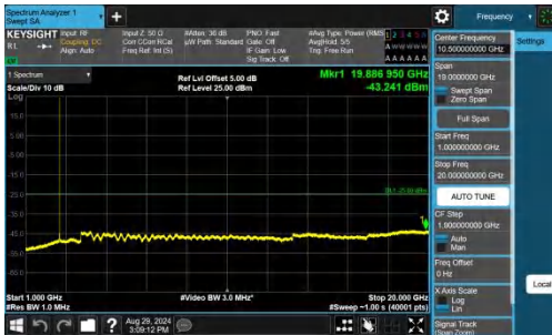
Band38-5MHz-QPSK-38000-1RB#24-1000~20000-PASS
