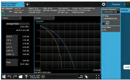
Band38-5MHz-QPSK-38000-25RB#0-PASS
