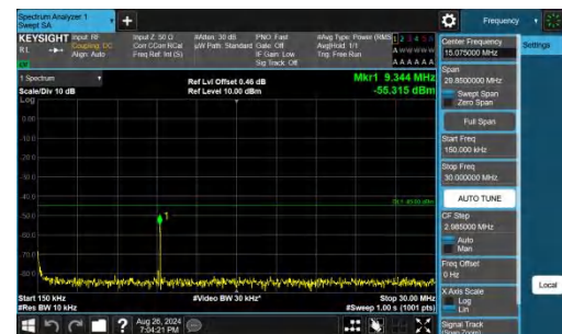
Band38-10MHz-QPSK-37800-1RB#0-0.15~30-PASS
