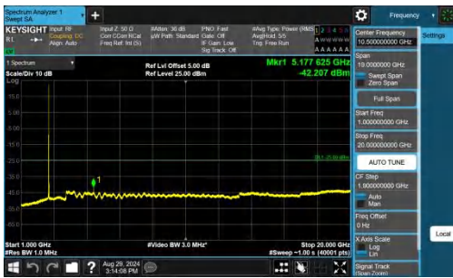
Band38-20MHz-QPSK-37850-1RB#99-1000~20000-PASS
