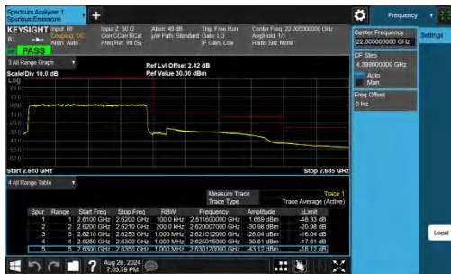
Band38-10MHz-QPSK-38200-50RB#0-PASS
