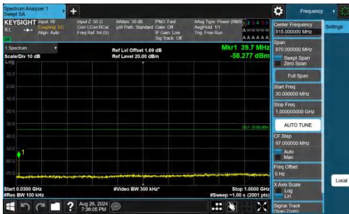
Band38-20MHz-QPSK-38150-1RB#0-30~1000-PASS
