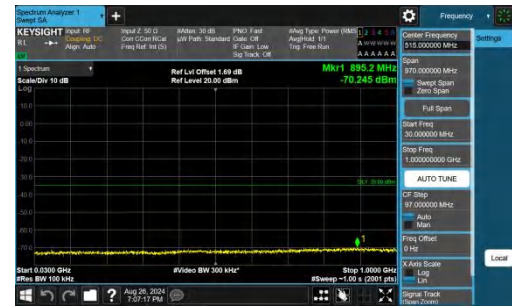
Band38-10MHz-QPSK-38200-1RB#49-30~1000-PASS
