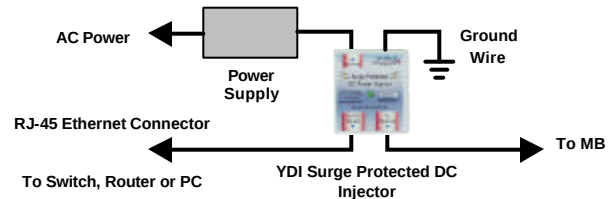
Figure 8 – Installation of the Optional YDI Surge Protected DC Injector
