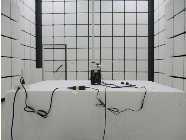
FCC_15_225_NFC_Radiated_Setup
