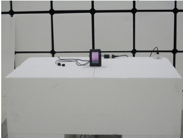
FCC_15_225_NFC_Radiated_Setup
