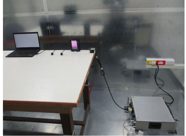
FCC_15_225_NFC_Conduction_Setup
