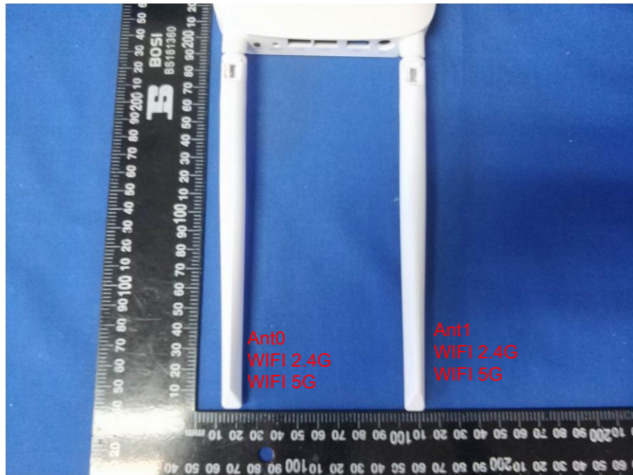
Antenna View
