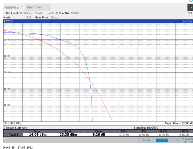
Band26-5MHz-QPSK-26740-6RB#0
