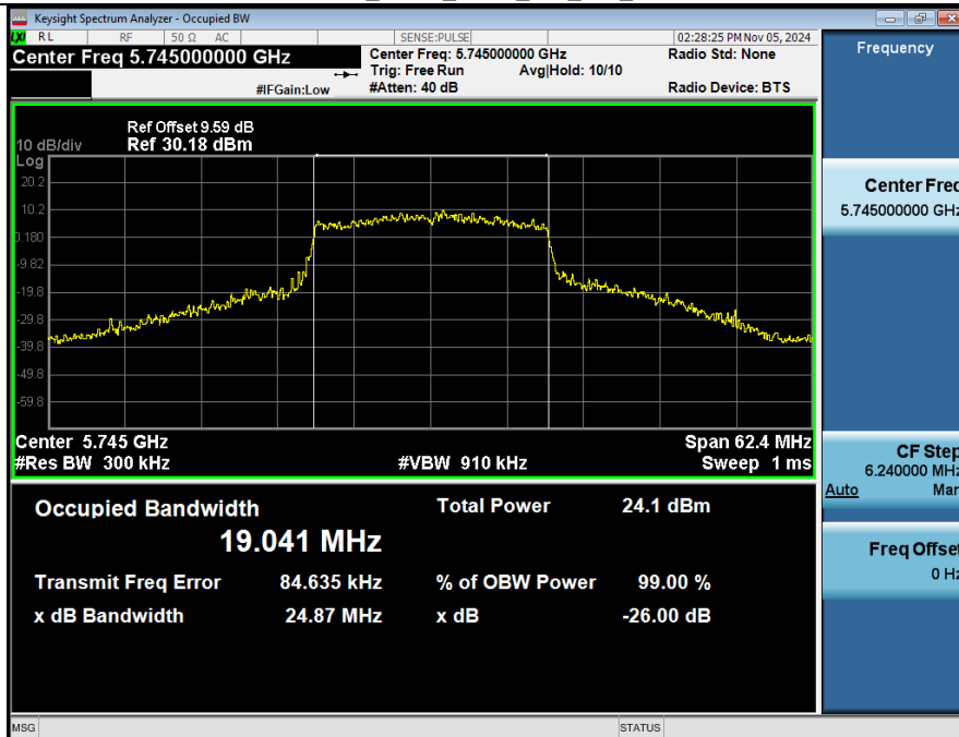
99%_OCB_NVNT_ANT2_802_11a_5745
