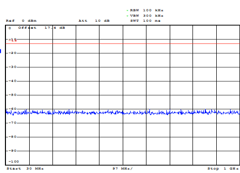
WCDMA Band IV CH-Middle 30MHz~1GHz
