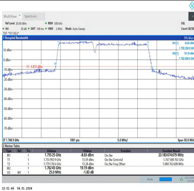
66-66-10MHz-15MHz-64QAM-64QAM-132477-132597-50RB #0-75RB#0-PASS
