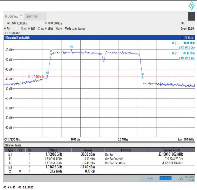
66-66-15MHz-10MHz-16QAM-16QAM-132047-132167-75RB #0-50RB#0-PASS
