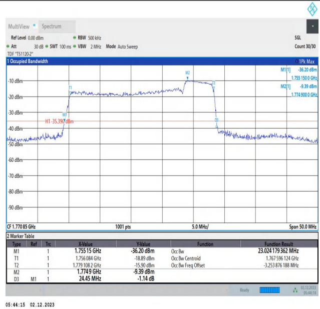
66-66-20MHz-5MHz-QPSK-QPSK-132522-132639-100RB#0 -25RB#0-PASS
