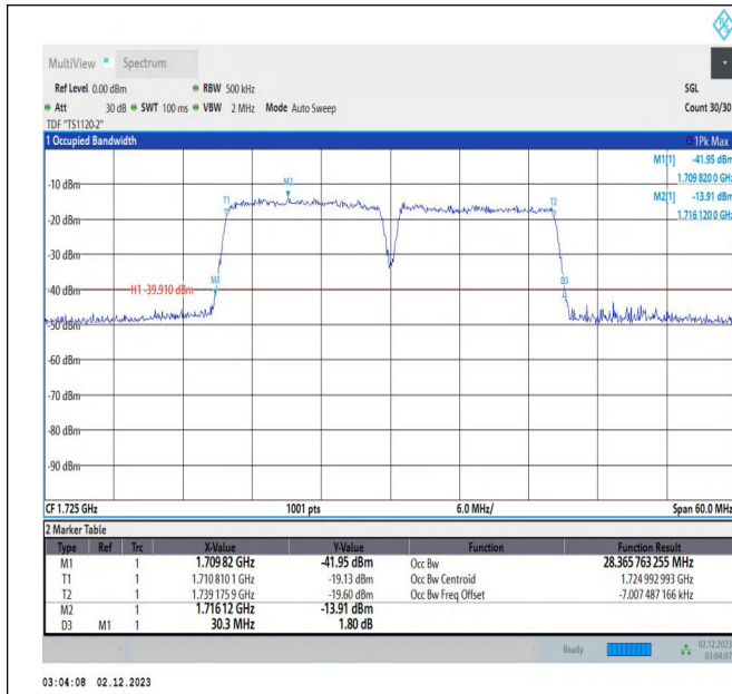
66-66-15MHz-15MHz-16QAM-16QAM-132047-132197-75RB #0-75RB#0-PASS
