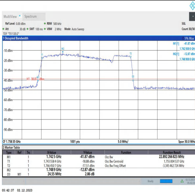
66-66-20MHz-5MHz-16QAM-16QAM-132397-132514-100RB #0-25RB#0-PASS
