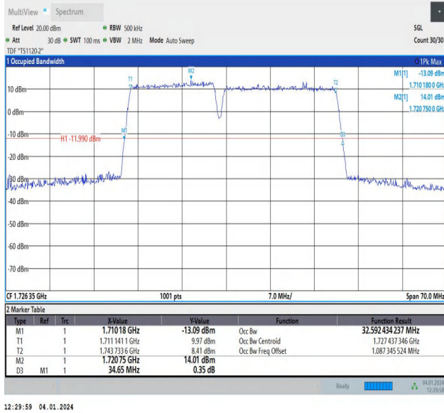
66-66-15MHz-20MHz-64QAM-64QAM-132050-132221-75RB #0-100RB#0-PASS
