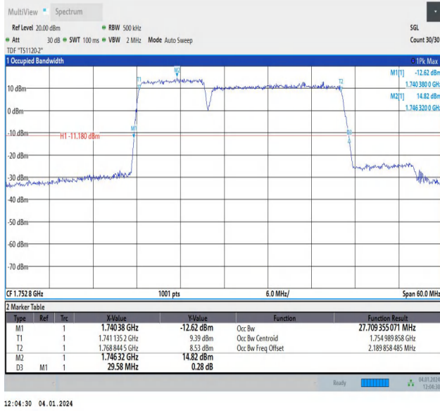
66-66-10MHz-20MHz-64QAM-64QAM-132328-132472-50RB #0-100RB#0-PASS
