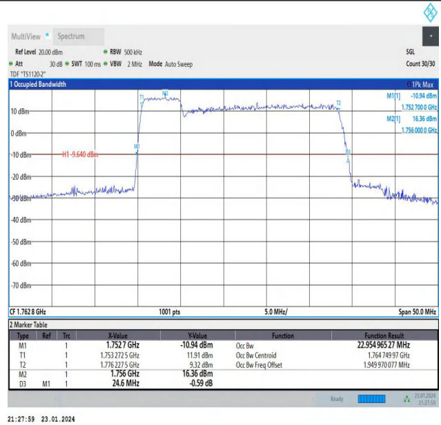
66-66-5MHz-20MHz-16QAM-16QAM-132428-132572-25RB# 0-100RB#0-PASS
