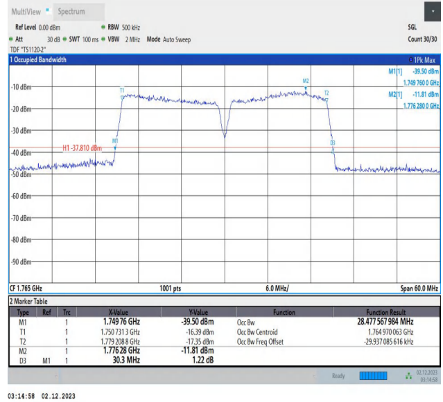
66-66-15MHz-15MHz-QPSK-QPSK-132447-132597-75RB#0 -75RB#0-PASS
