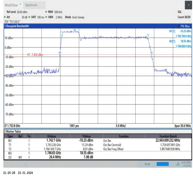
66-66-5MHz-20MHz-64QAM-64QAM-132328-132472-25RB# 0-100RB#0-PASS
