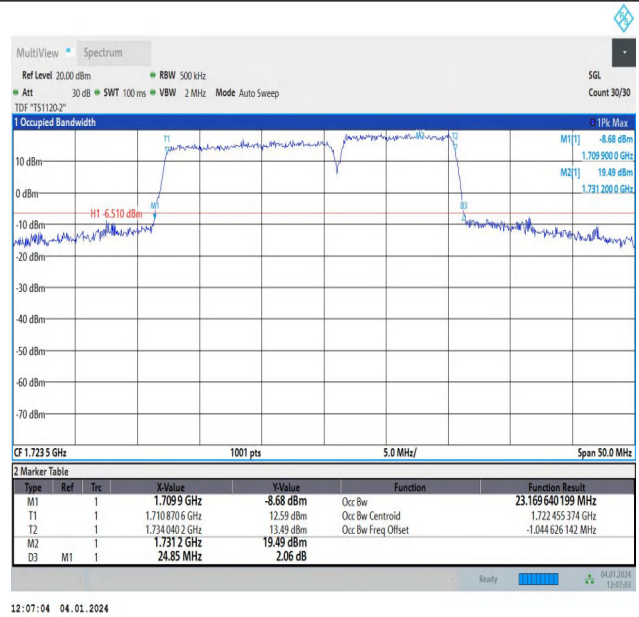
66-66-15MHz-10MHz-64QAM-64QAM-132047-132167-75RB #0-50RB#0-PASS
