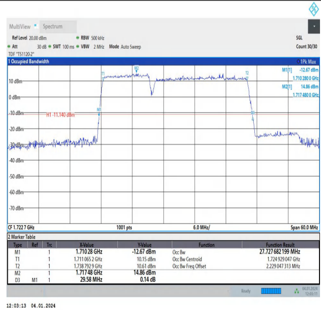
66-66-10MHz-20MHz-64QAM-64QAM-132027-132171-50RB #0-100RB#0-PASS
