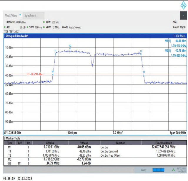
66-66-15MHz-20MHz-QPSK-QPSK-132050-132221-75RB#0 -100RB#0-PASS
