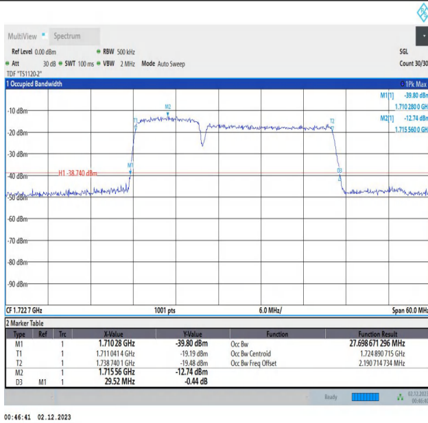
66-66-10MHz-20MHz-16QAM-16QAM-132027-132171-50RB #0-100RB#0-PASS
