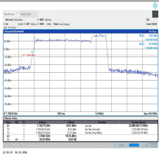
66-66-20MHz-5MHz-64QAM-64QAM-132397-132514-100RB #0-25RB#0-PASS
