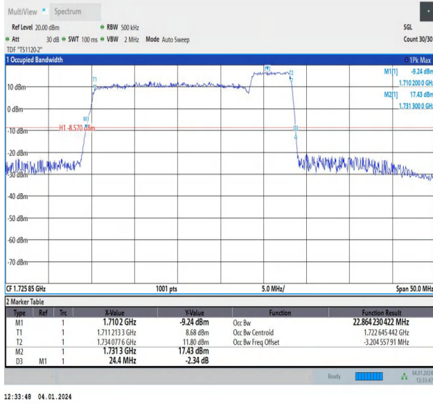
66-66-20MHz-5MHz-64QAM-64QAM-132072-132189-100RB #0-25RB#0-PASS
