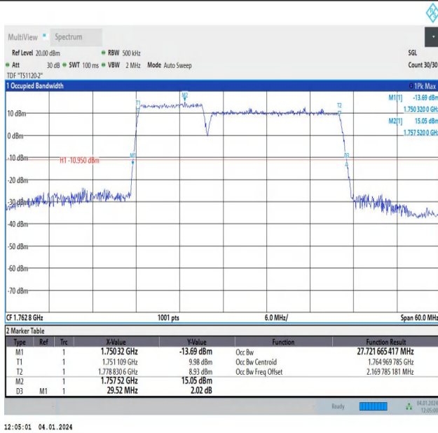
66-66-10MHz-20MHz-64QAM-64QAM-132428-132572-50RB #0-100RB#0-PASS
