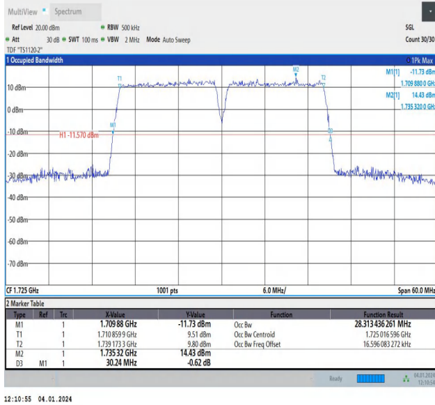
66-66-15MHz-15MHz-64QAM-64QAM-132047-132197-75RB #0-75RB#0-PASS
