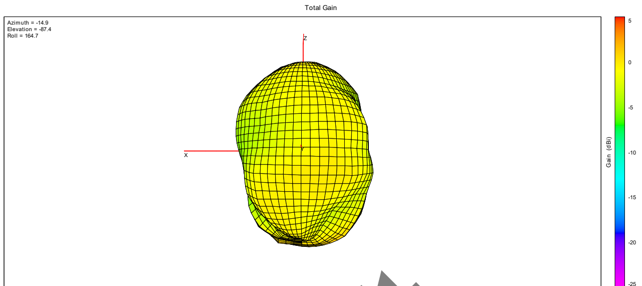
2480MHz_C4207-810023-A(SSR-2400194)-X3
