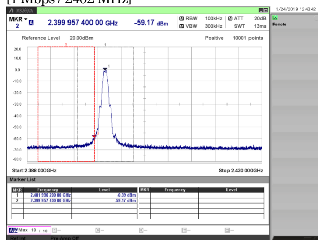
[1 Mbps / 2402 MHz]
