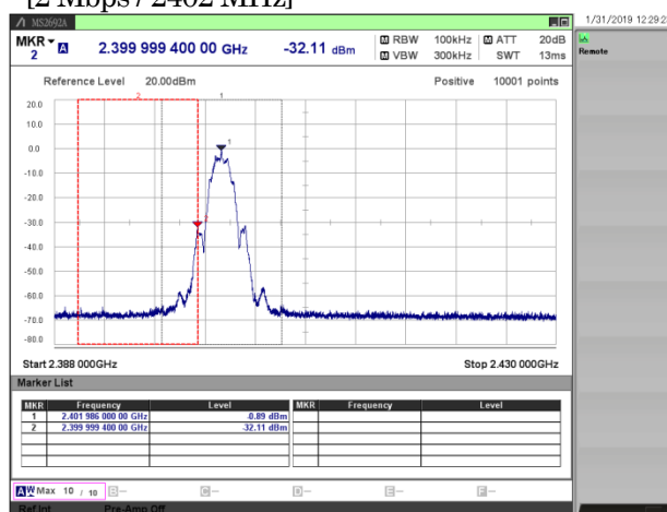
[2 Mbps / 2402 MHz]
