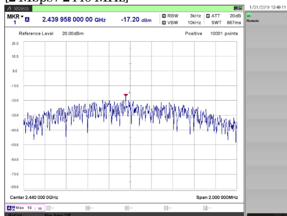
[2 Mbps / 2440 MHz]
