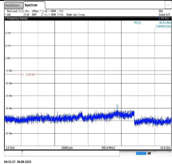
Band12-10MHz-QPSK-23060-1RB#0- Range2:1000~10000MHz
