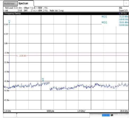
Band25-1.4MHz-16QAM-26365-1RB#0- Range2:1000~20000MHz
