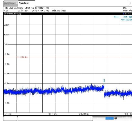
Band17-10MHz-QPSK-23780-1RB#0- Range2:1000~10000MHz
