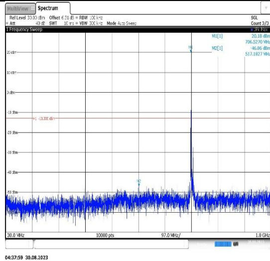
Band17-5MHz-QPSK-23755-1RB#0- Range1:30~1000MHz
