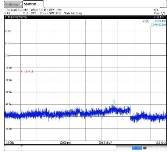
Band17-5MHz-16QAM-23755-1RB#0- Range2:1000~10000MHz
