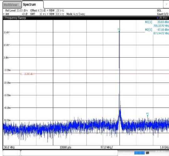
Band17-10MHz-QPSK-23790-1RB#0- Range1:30~1000MHz
