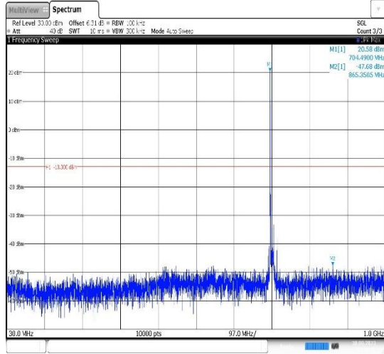
Band17-10MHz-QPSK-23780-1RB#0- Range1:30~1000MHz
