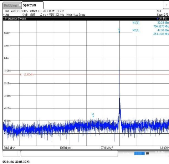
Band17-10MHz-16QAM-23780-1RB#0- Range1:30~1000MHz
