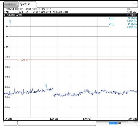
Band25-1.4MHz-16QAM-26047-1RB#0- Range2:1000~20000MHz
