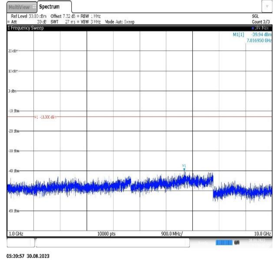
Band17-10MHz-16QAM-23790-1RB#0- Range2:1000~10000MHz
