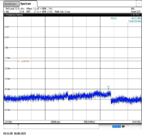
Band17-10MHz-16QAM-23800-1RB#0- Range2:1000~10000MHz
