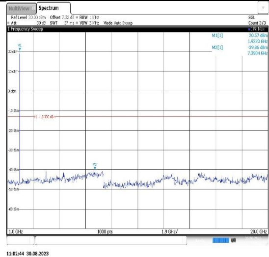
Band25-3MHz-16QAM-26055-1RB#0- Range2:1000~20000MHz
