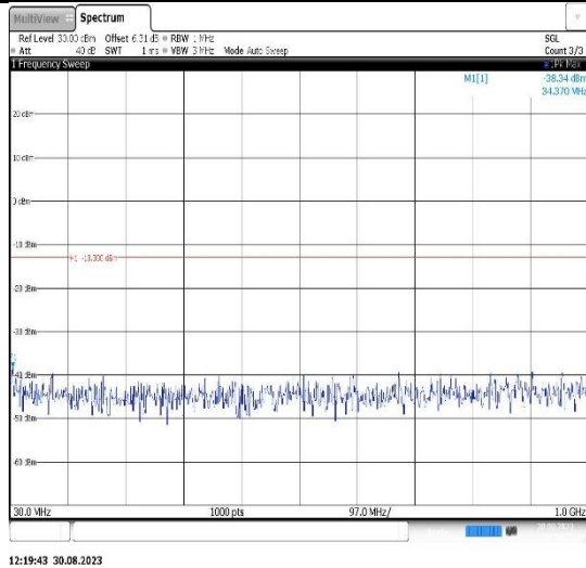
Band25-15MHz-16QAM-26115-1RB#0- Range1:30~1000MHz
