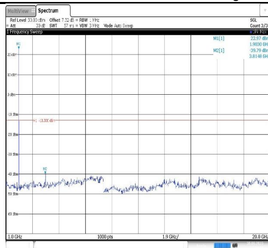
Band25-5MHz-16QAM-26065-1RB#0- Range2:1000~20000MHz
