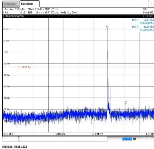
Band12-10MHz-QPSK-23095-1RB#0- Range1:30~1000MHz
