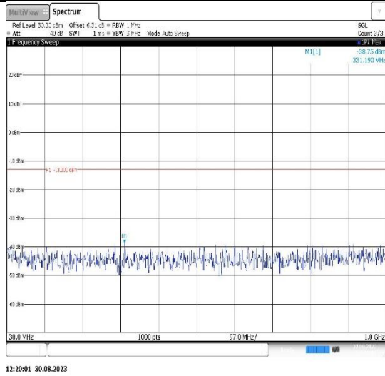
Band25-20MHz-QPSK-26140-1RB#0- Range1:30~1000MHz
