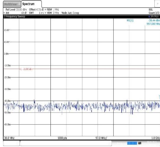
Band25-1.4MHz-16QAM-26047-1RB#0- Range1:30~1000MHz
