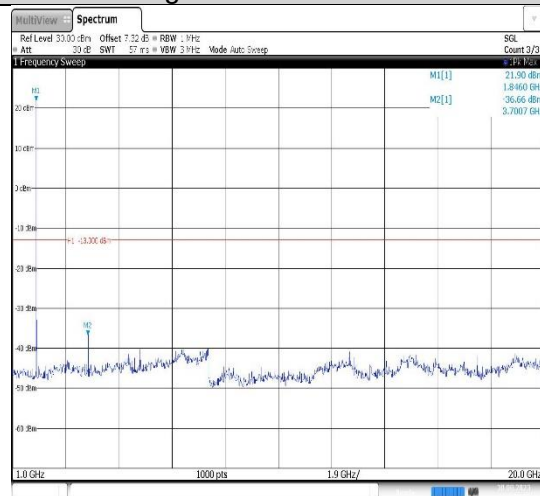
Band25-5MHz-16QAM-26065-1RB#0- Range2:1000~20000MHz
