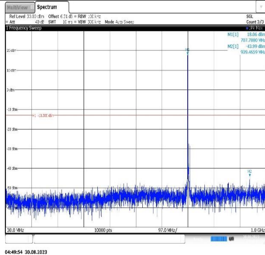
Band17-5MHz-QPSK-23825-1RB#0- Range1:30~1000MHz
