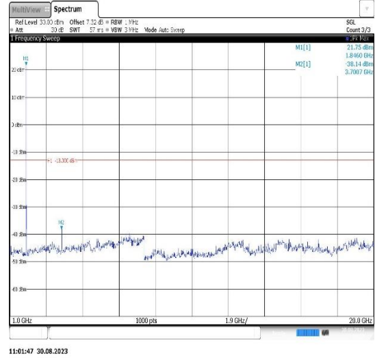
Band25-3MHz-16QAM-26365-1RB#0- Range2:1000~20000MHz
