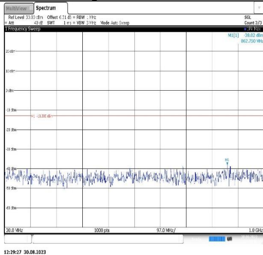
Band25-20MHz-QPSK-26590-1RB#0- Range1:30~1000MHz
