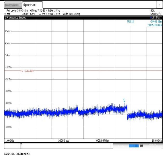
Band17-10MHz-16QAM-23780-1RB#0- Range2:1000~10000MHz
