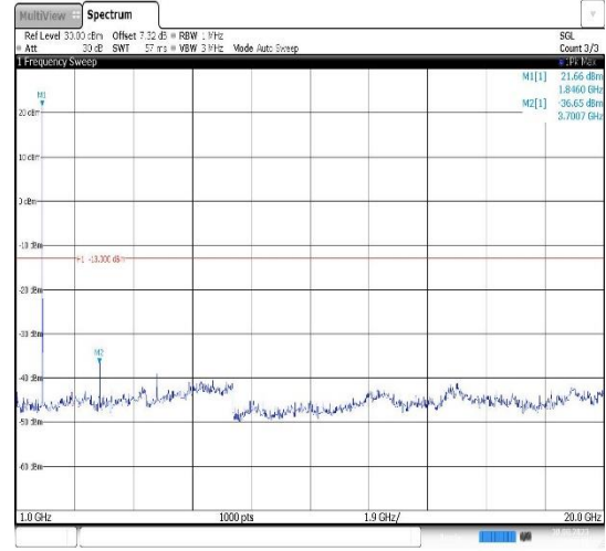
Band25-10MHz-16QAM-26090-1RB#0- Range2:1000~20000MHz
