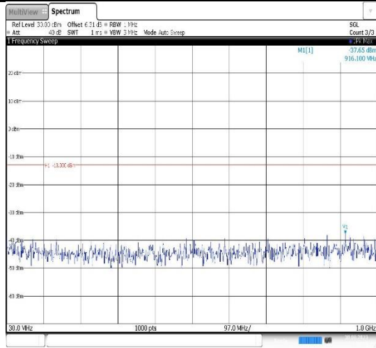
Band25-5MHz-QPSK-26065-1RB#0- Range1:30~1000MHz
