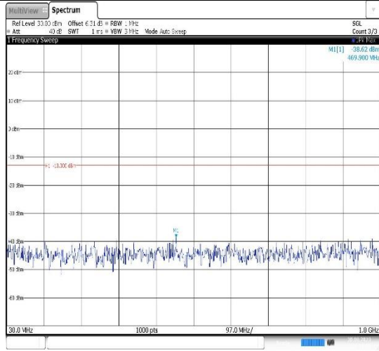
Band25-15MHz-QPSK-26365-1RB#0- Range1:30~1000MHz
