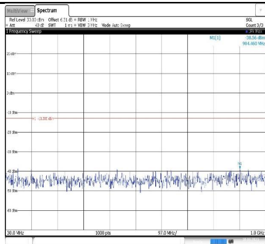
Band25-5MHz-16QAM-26065-1RB#0- Range1:30~1000MHz
