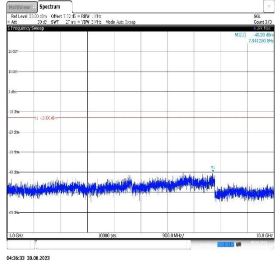
Band12-10MHz-QPSK-23095-1RB#0- Range2:1000~10000MHz
