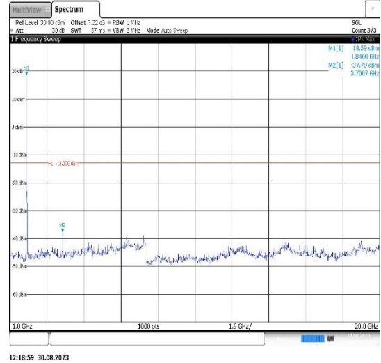
Band25-15MHz-16QAM-26365-1RB#0- Range2:1000~20000MHz
