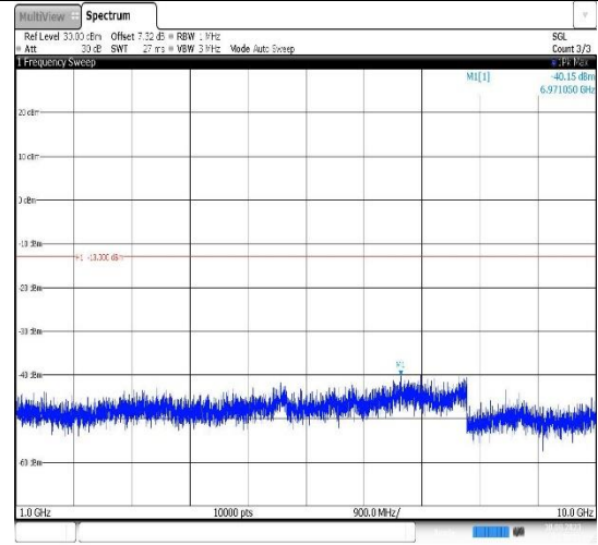
Band17-5MHz-16QAM-23790-1RB#0- Range2:1000~10000MHz
