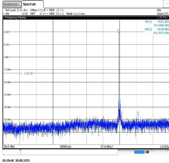
Band17-10MHz-16QAM-23790-1RB#0- Range1:30~1000MHz
