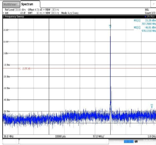
Band17-5MHz-16QAM-23790-1RB#0- Range1:30~1000MHz
