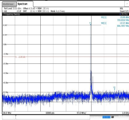
Band12-10MHz-16QAM-23095-1RB#0- Range1:30~1000MHz
