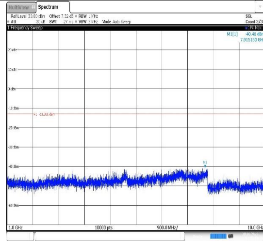
Band17-10MHz-QPSK-23790-1RB#0- Range2:1000~10000MHz
