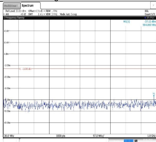
Band25-5MHz-16QAM-26065-1RB#0- Range1:30~1000MHz
