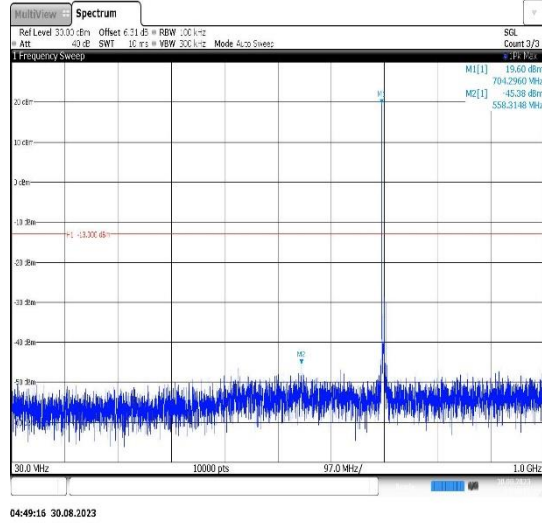
Band17-5MHz-QPSK-23790-1RB#0- Range1:30~1000MHz
