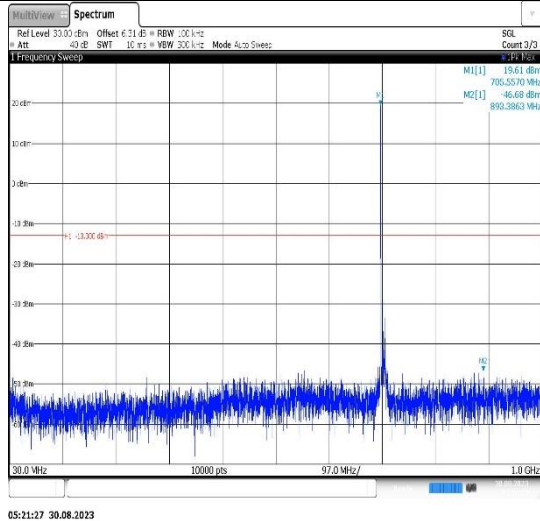
Band17-10MHz-16QAM-23800-1RB#0- Range1:30~1000MHz
