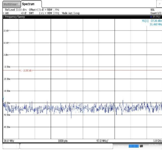
Band25-10MHz-QPSK-26090-1RB#0- Range1:30~1000MHz
