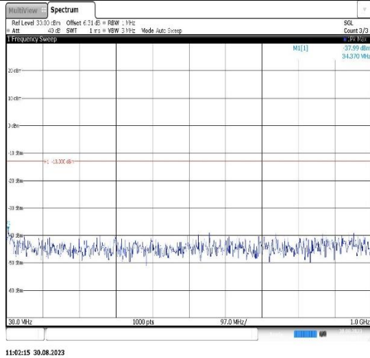
Band25-3MHz-16QAM-26675-1RB#0- Range1:30~1000MHz
