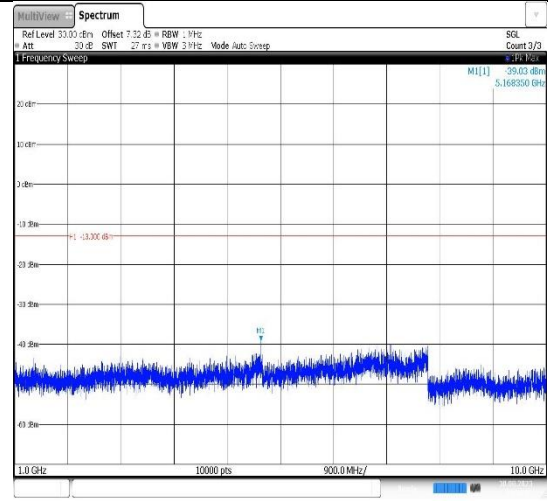
Band12-10MHz-16QAM-23060-1RB#0- Range2:1000~10000MHz
