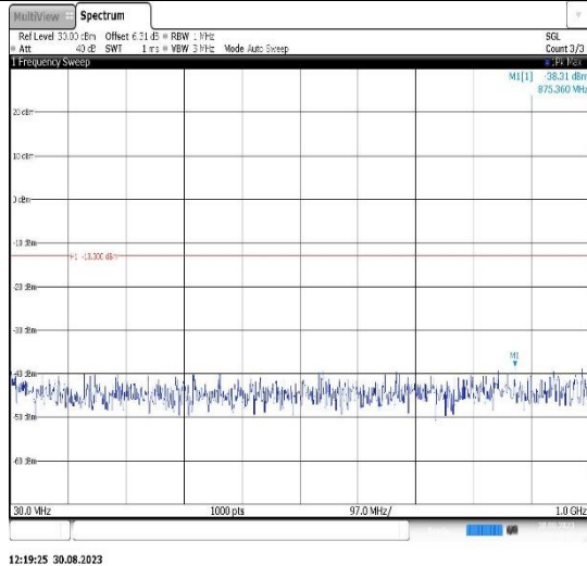
Band25-15MHz-16QAM-26615-1RB#0- Range1:30~1000MHz
