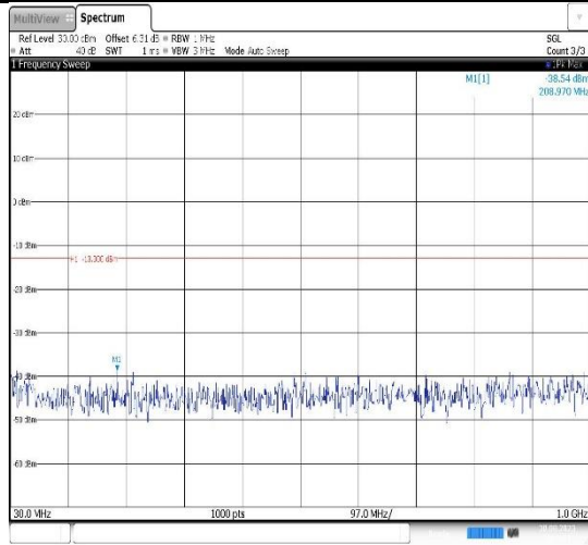
Band25-3MHz-QPSK-26055-1RB#0- Range1:30~1000MHz
