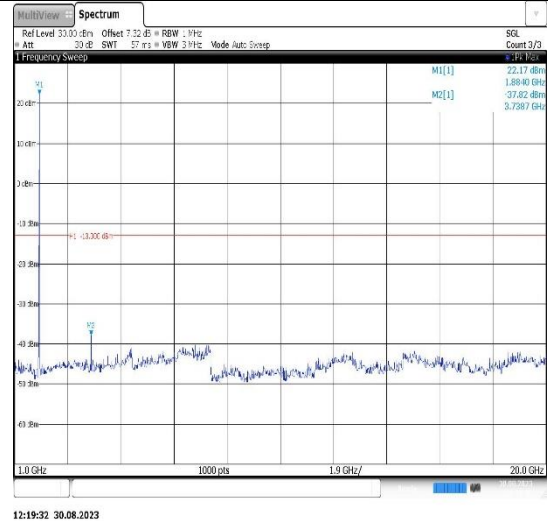
Band25-15MHz-16QAM-26615-1RB#0- Range2:1000~20000MHz
