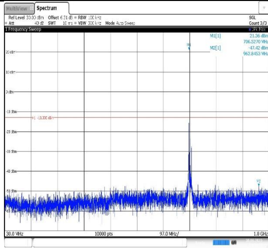
Band12-10MHz-16QAM-23060-1RB#0- Range1:30~1000MHz
