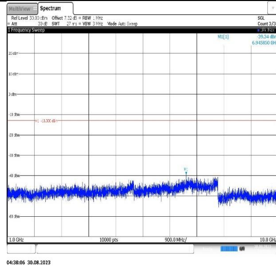
Band17-5MHz-QPSK-23755-1RB#0- Range2:1000~10000MHz
