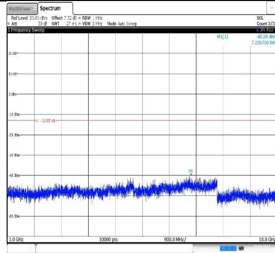
Band17-10MHz-QPSK-23780-1RB#0- Range2:1000~10000MHz
