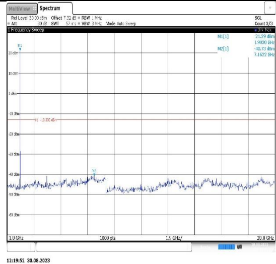
Band25-15MHz-16QAM-26115-1RB#0- Range2:1000~20000MHz
