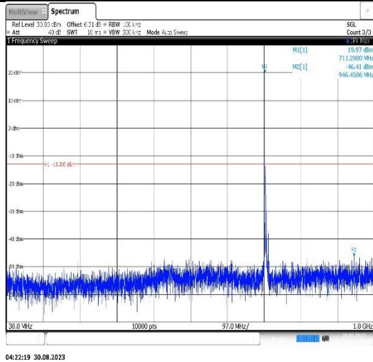
Band12-10MHz-QPSK-23060-1RB#0- Range1:30~1000MHz
