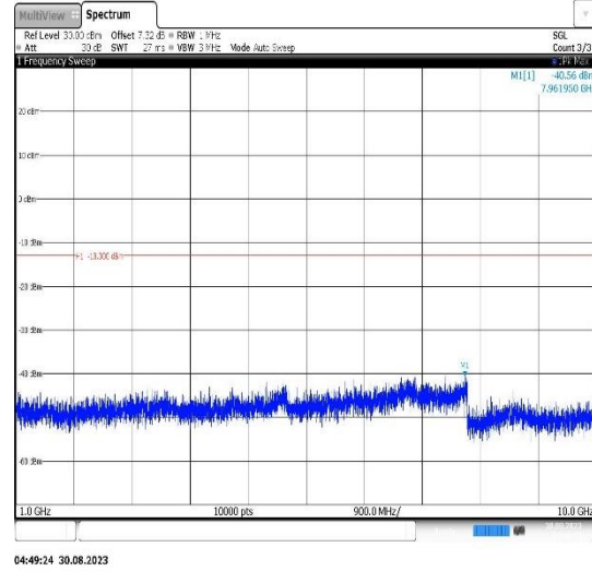
Band17-5MHz-QPSK-23790-1RB#0- Range2:1000~10000MHz
