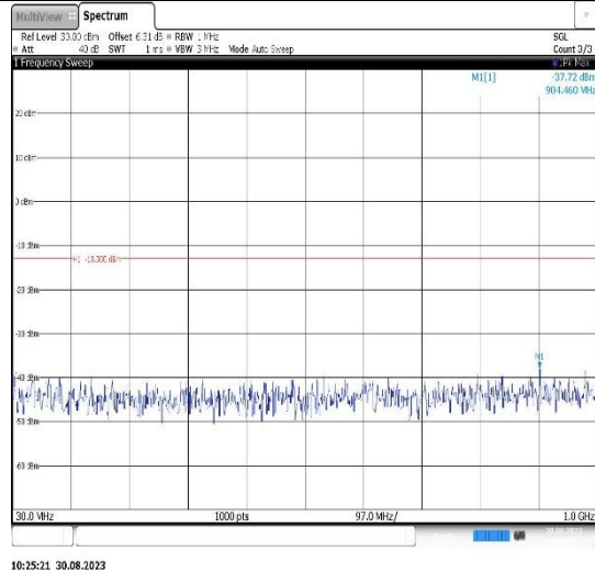
Band25-1.4MHz-QPSK-26683-1RB#0- Range1:30~1000MHz
