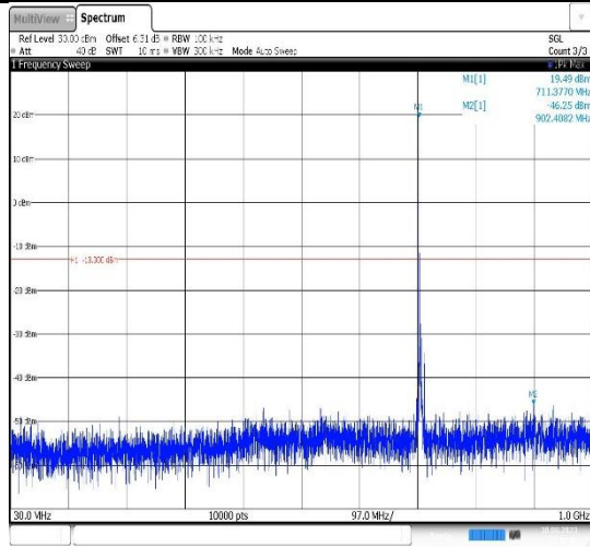
Band17-5MHz-16QAM-23755-1RB#0- Range1:30~1000MHz
