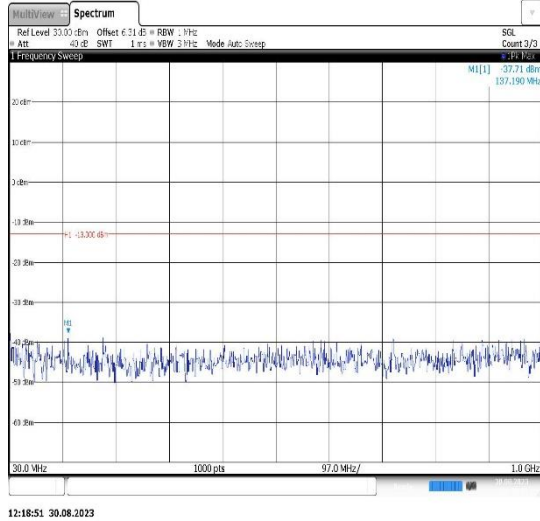
Band25-15MHz-16QAM-26365-1RB#0- Range1:30~1000MHz
