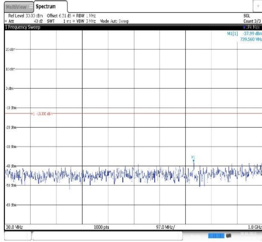
Band25-10MHz-16QAM-26090-1RB#0- Range1:30~1000MHz
