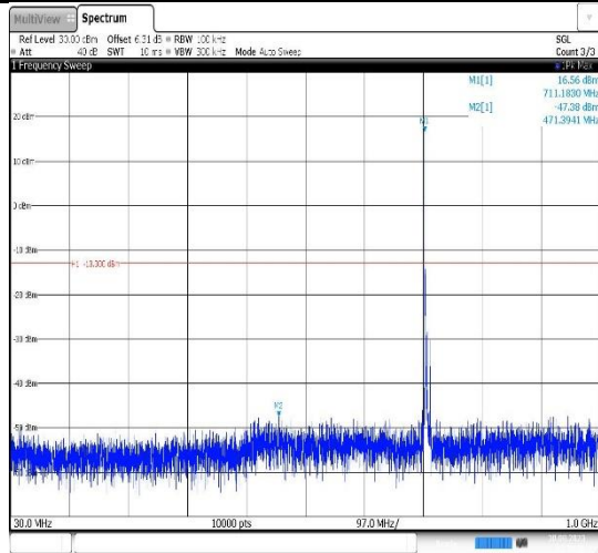
Band17-10MHz-QPSK-23780-1RB#0- Range1:30~1000MHz
