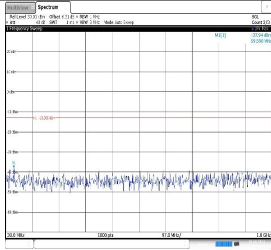
Band25-1.4MHz-16QAM-26365-1RB#0- Range1:30~1000MHz
