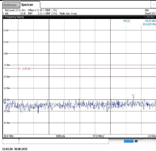
Band25-3MHz-16QAM-26055-1RB#0- Range1:30~1000MHz
