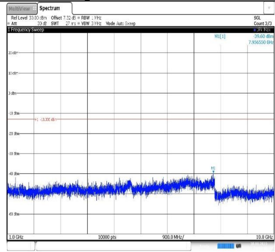
Band12-10MHz-16QAM-23095-1RB#0- Range2:1000~10000MHz
