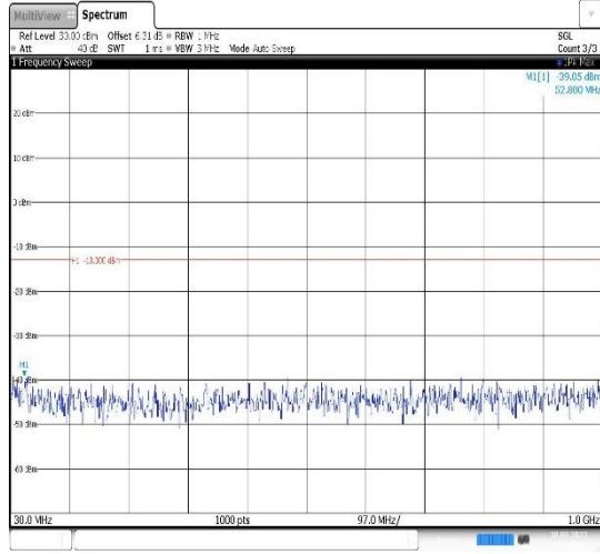
Band25-15MHz-QPSK-26115-1RB#0- Range1:30~1000MHz
