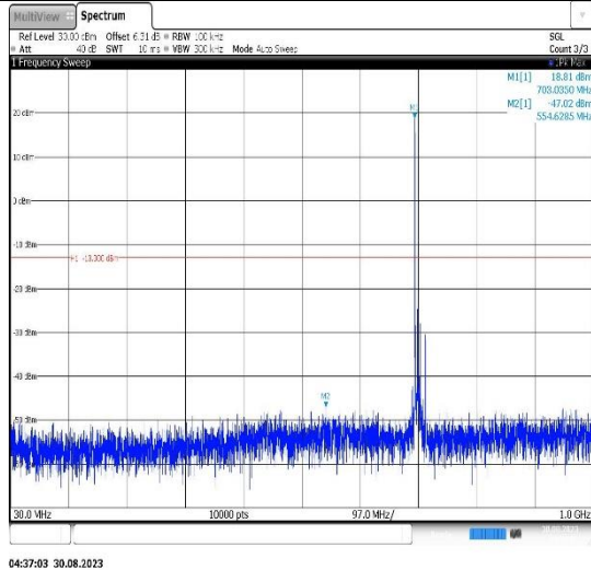
Band12-10MHz-QPSK-23130-1RB#0- Range1:30~1000MHz
