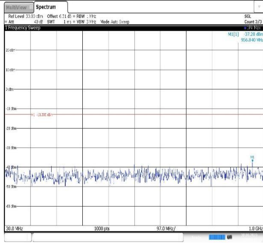
Band25-10MHz-16QAM-26365-1RB#0- Range1:30~1000MHz
