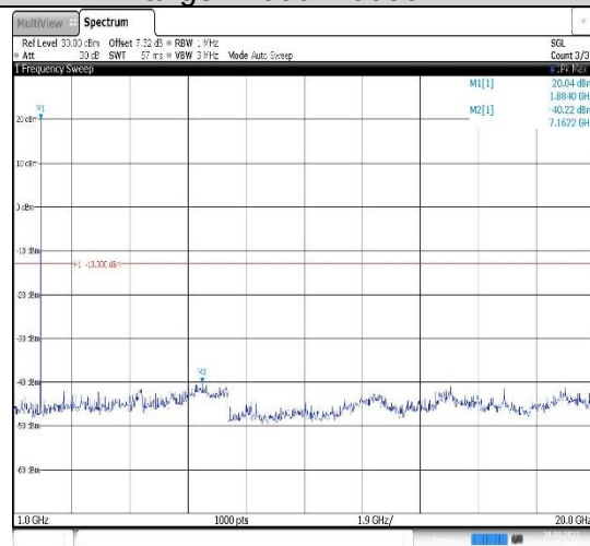
Band25-5MHz-16QAM-26365-1RB#0- Range2:1000~20000MHz
