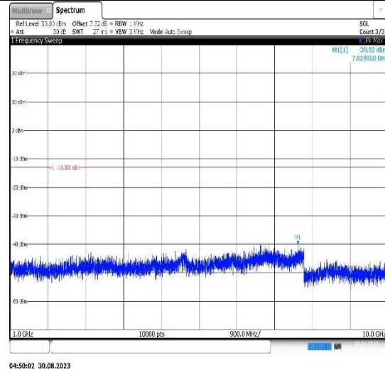
Band17-5MHz-QPSK-23825-1RB#0- Range2:1000~10000MHz
