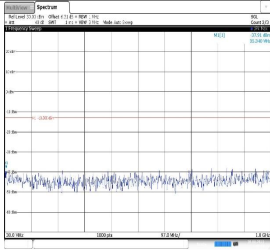
Band25-3MHz-QPSK-26365-1RB#0- Range1:30~1000MHz
