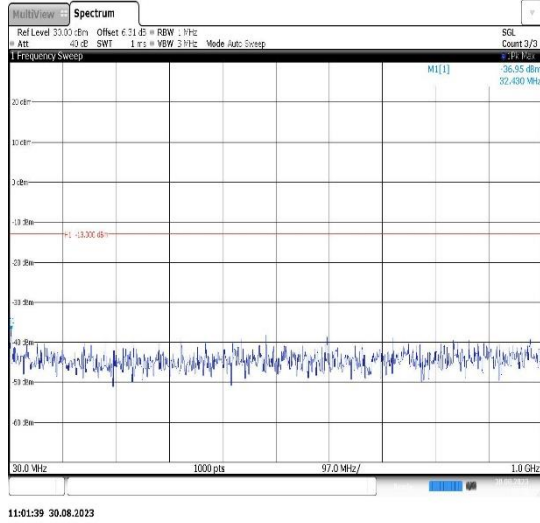
Band25-3MHz-16QAM-26365-1RB#0- Range1:30~1000MHz
