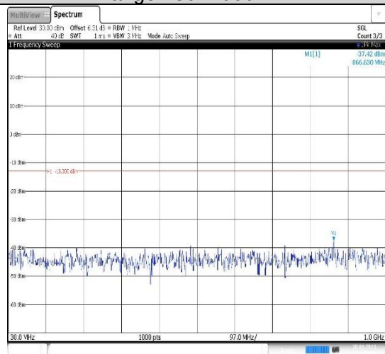
Band25-5MHz-16QAM-26365-1RB#0- Range1:30~1000MHz
