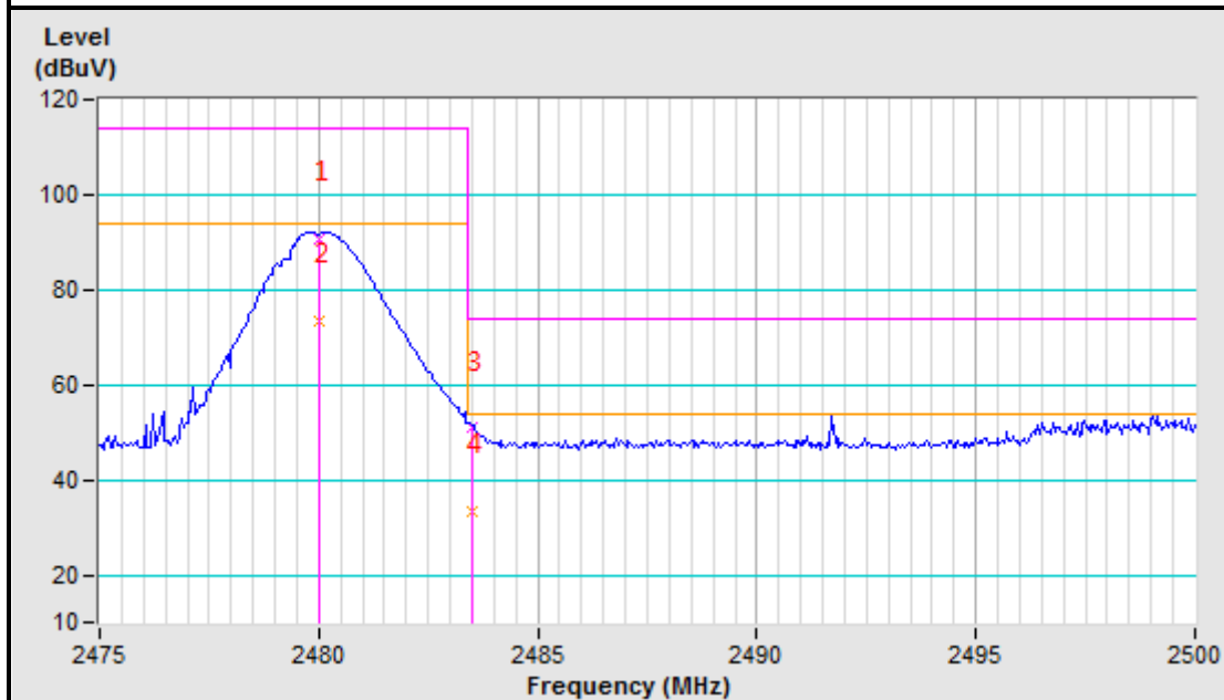
2480MHz Vertical
