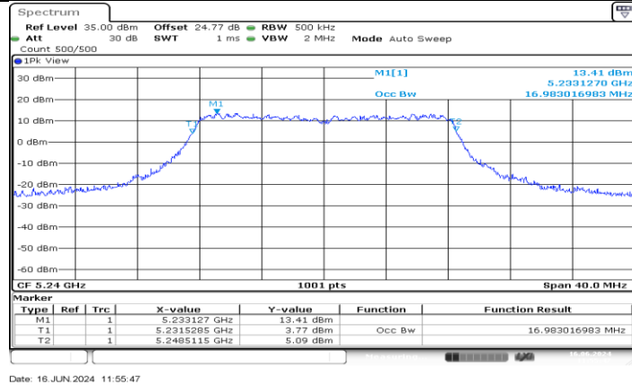
11A-CDD_Ant4_5240
